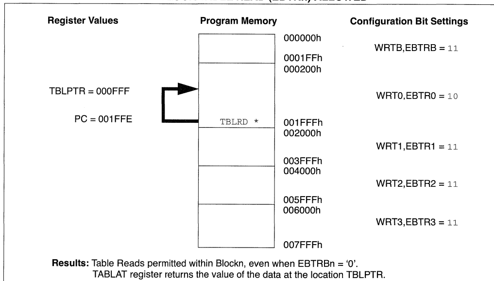
FIGURE 24-6: EXTERNAL BLOCK TABLE READ (EBTRn) ALLOWED
