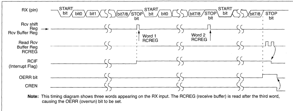
FIGURE 18-5: ASYNCHRONOUS RECEPTION
