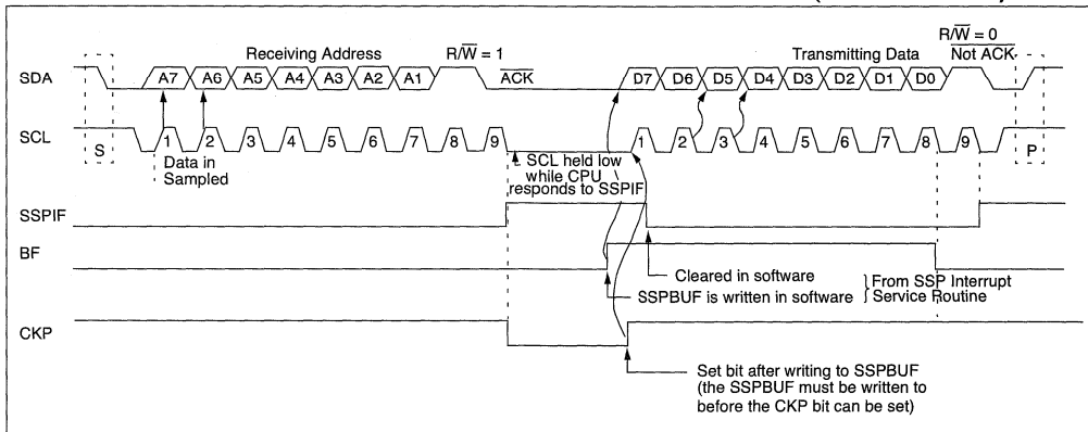
FIGURE 17-8: I 2 C SLAVE MODE WAVEFORMS FOR TRANSMISSION (7-BIT ADDRESS)
