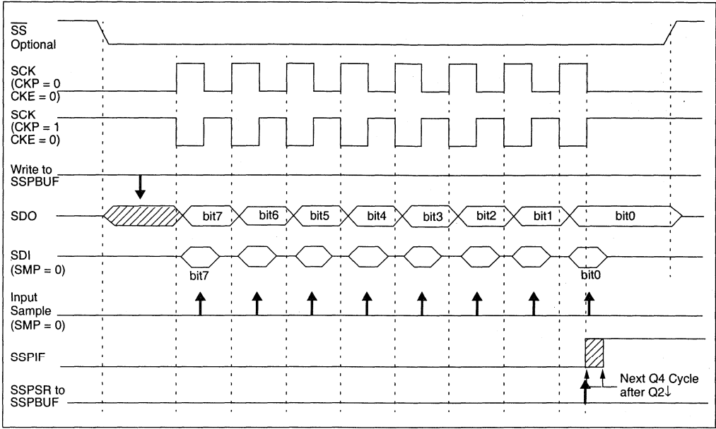
FIGURE 17-4: SPI MODE WAVEFORM (SLAVE MODE WITH CKE = 0)
