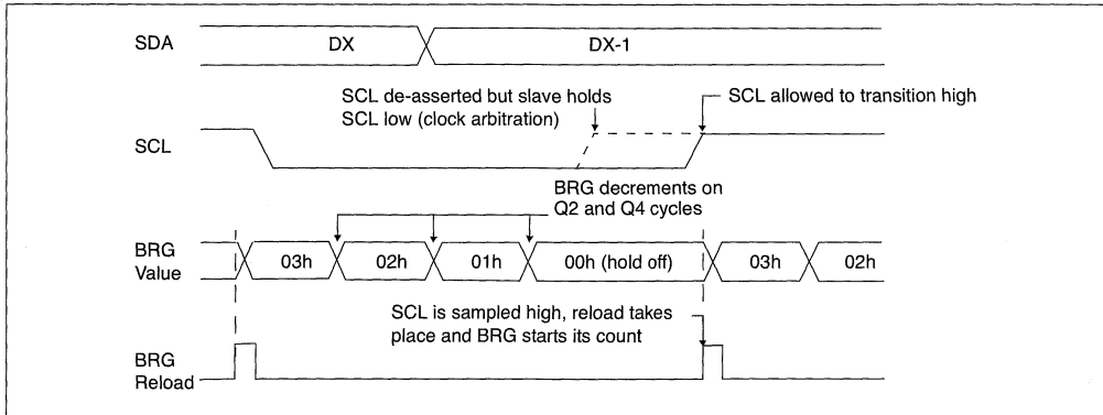
FIGURE 17-12: BAUD RATE GENERATOR TIMING WITH CLOCK ARBITRATION
