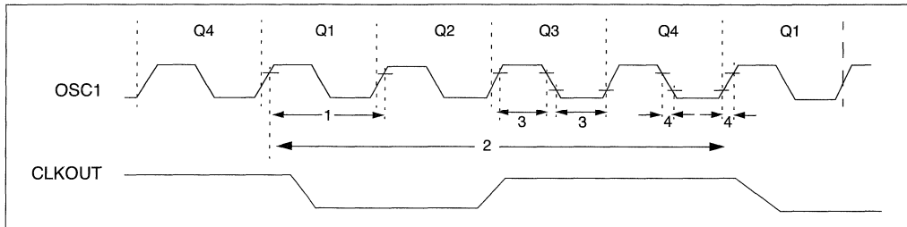
FIGURE 27-5: EXTERNAL CLOCK TIMING
