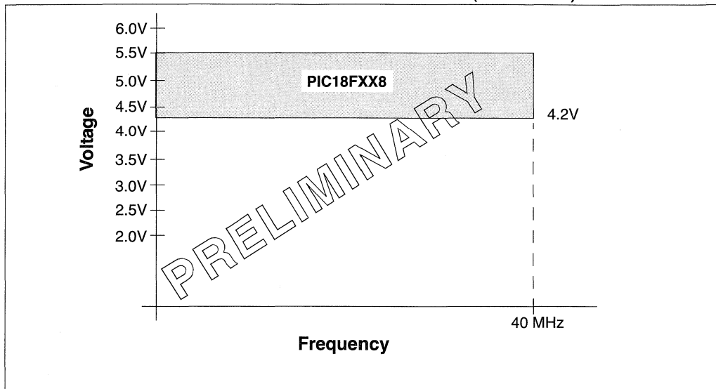
FIGURE 27-1: PIC18FXX8 VOLTAGE-FREQUENCY GRAPH (INDUSTRIAL)
