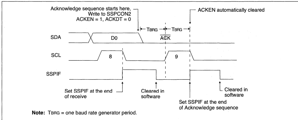
FIGURE 17-17: ACKNOWLEDGE SEQUENCE WAVEFORM
