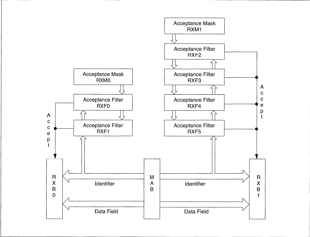
FIGURE 19-3: RECEIVE BUFFER BLOCK DIAGRAM
