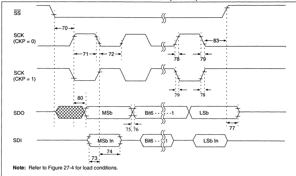
FIGURE 27-14: EXAMPLE SPI SLAVE MODE TIMING (CKE = 0)
