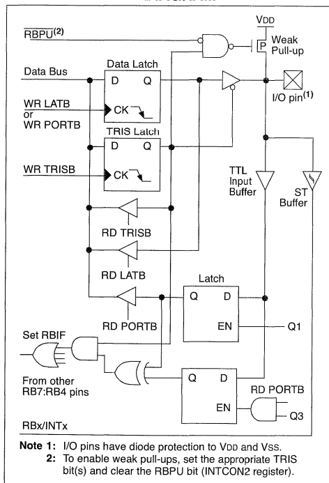
FIGURE 9-4: RB7:RB4 PINS BLOCK DIAGRAM
