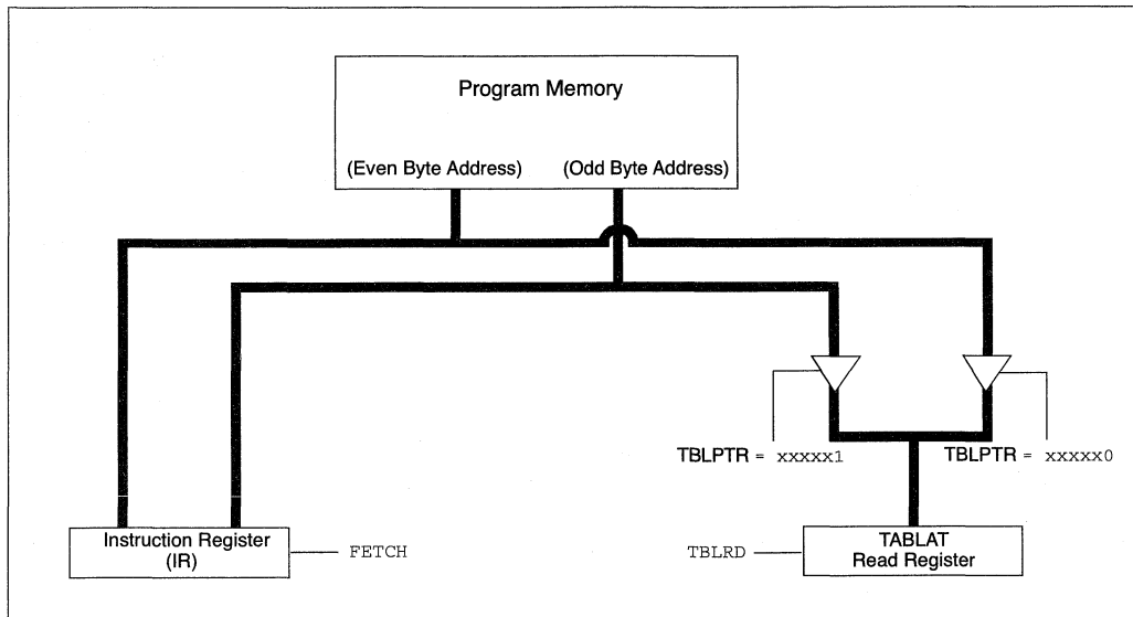
FIGURE 6-4: READS FROM FLASH PROGRAM MEMORY
