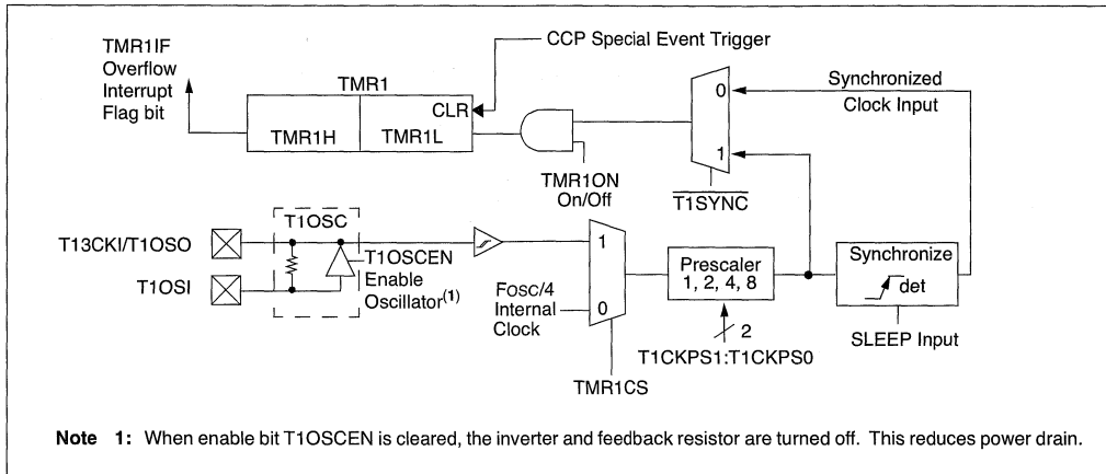
FIGURE 12-1: TIMER1 BLOCK DIAGRAM
