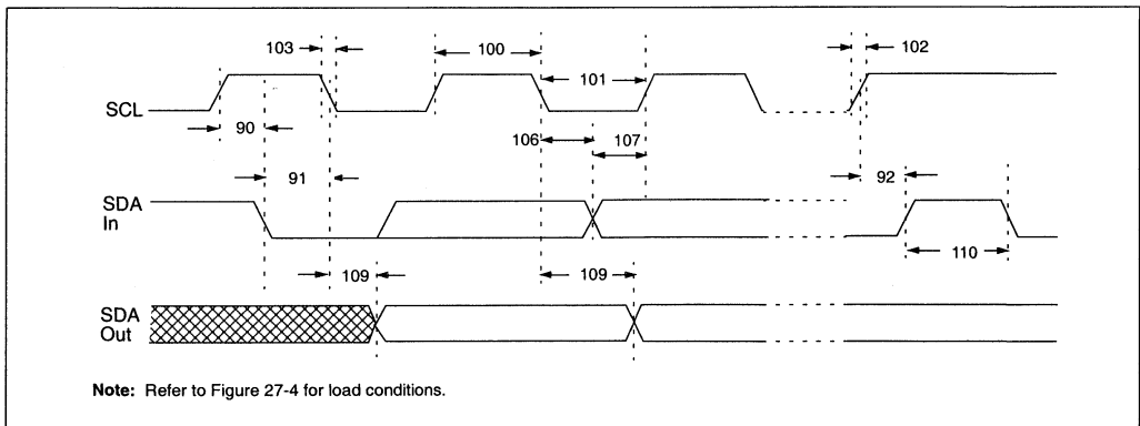
FIGURE 27-17: I 2 C BUS DATA TIMING
