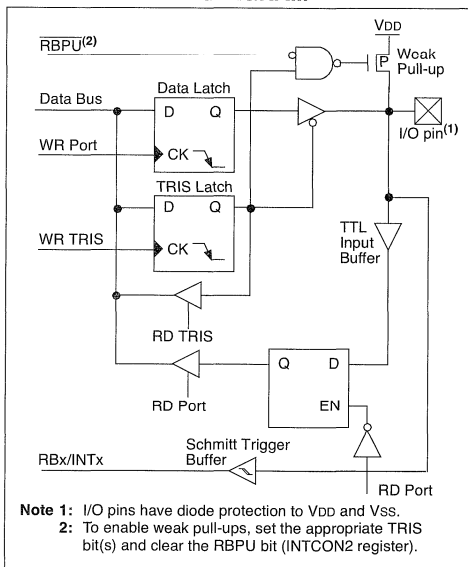
FIGURE 9-5: RB1:RB0 PINS BLOCK DIAGRAM
