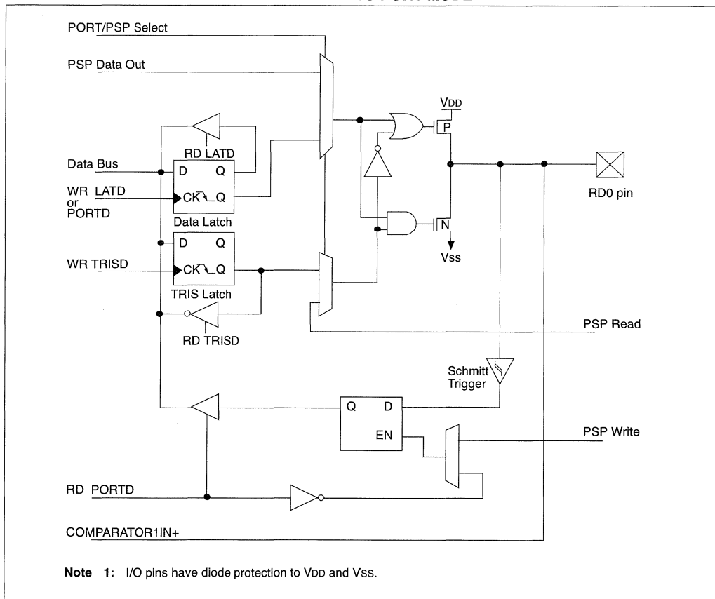
FIGURE 9-9: PORTD BLOCK DIAGRAM IN I/O PORT MODE
