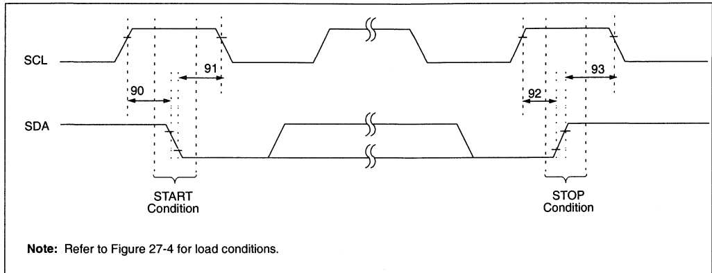
FIGURE 27-16: I 2 C BUS START/STOP BITS TIMING
