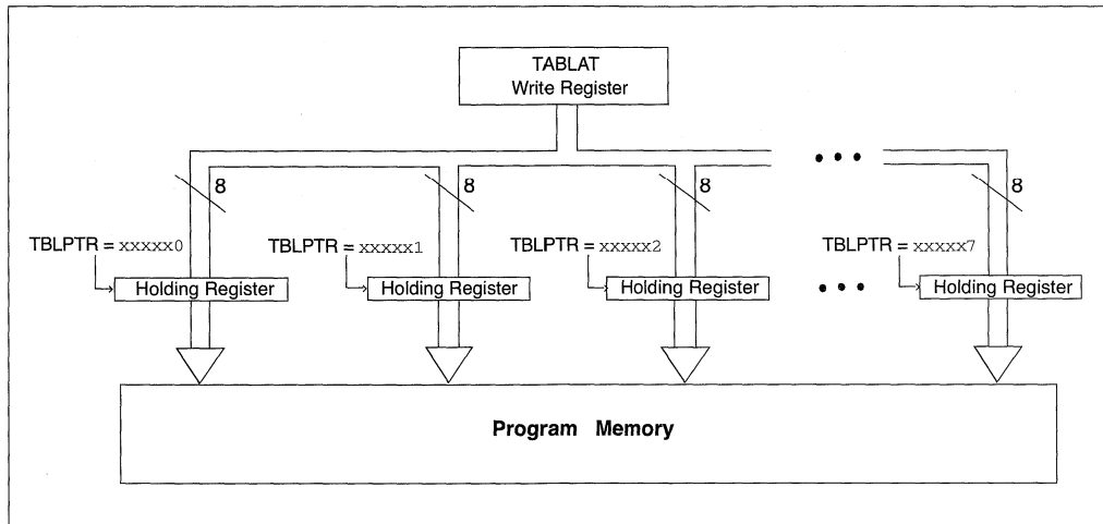
FIGURE 6-5: TABLE WRITES TO FLASH PROGRAM MEMORY
