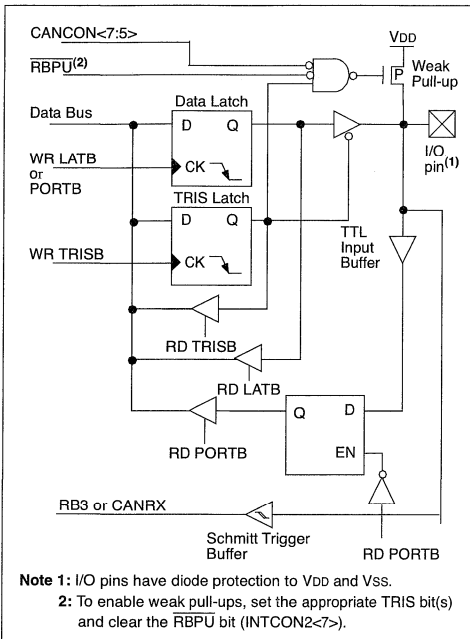
FIGURE 9-7: BLOCK DIAGRAM OF RB3/CANRX PIN
