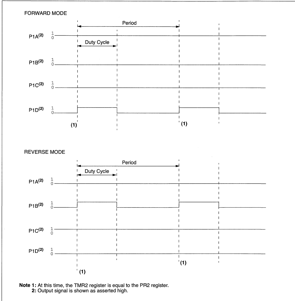
FIGURE 16-8: FULL-BRIDGE PWM OUTPUT
