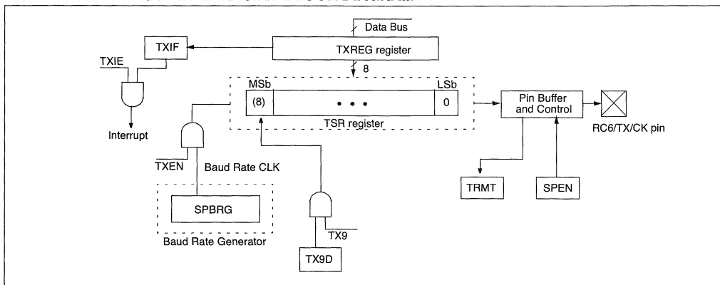
FIGURE 18-1: USART TRANSMIT BLOCK DIAGRAM
