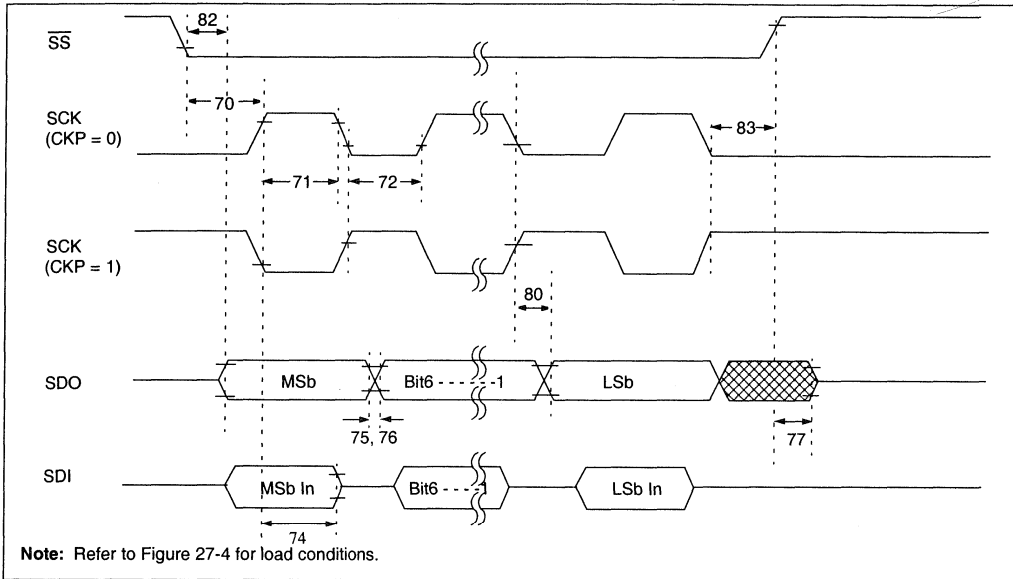
FIGURE 27-15: EXAMPLE SPI SLAVE MODE TIMING (CKE = 1)
