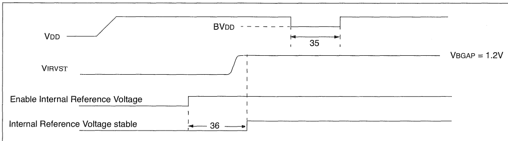
FIGURE 27-8: BROWN-OUT RESET TIMING
