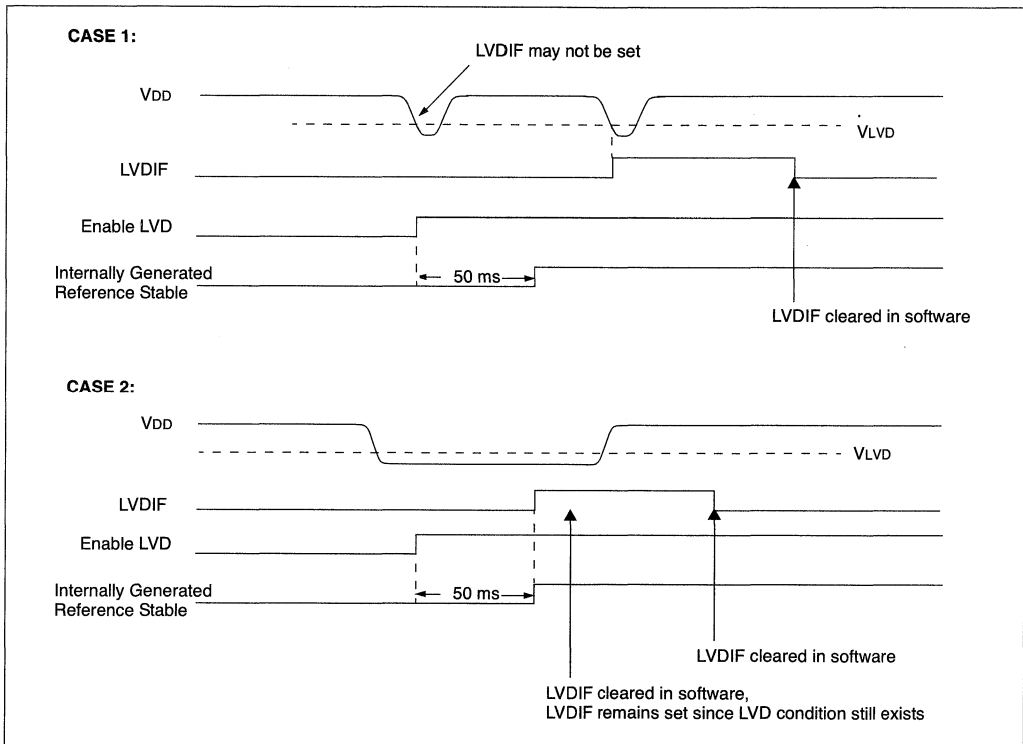
FIGURE 23-3: LOW VOLTAGE DETECT WAVEFORMS
