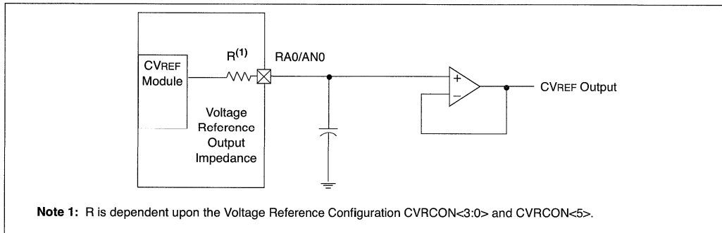
FIGURE 22-2: VOLTAGE REFERENCE OUTPUT BUFFER EXAMPLE
