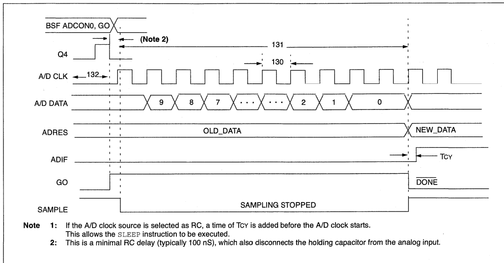
FIGURE 27-22: A/D CONVERSION TIMING
