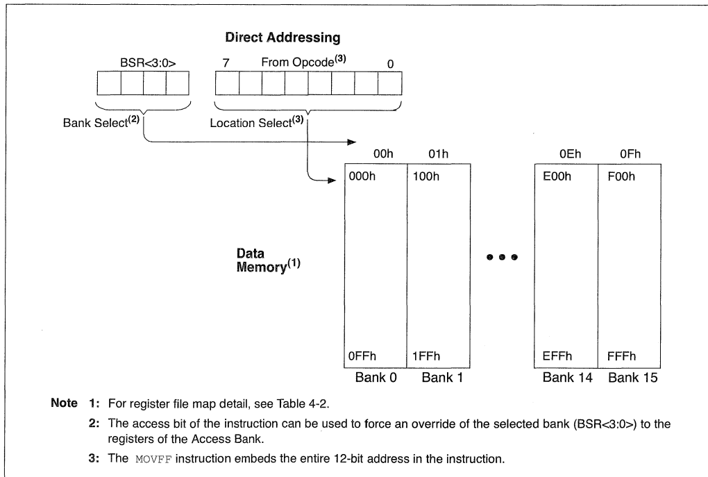
FIGURE 4-7: DIRECT ADDRESSING
