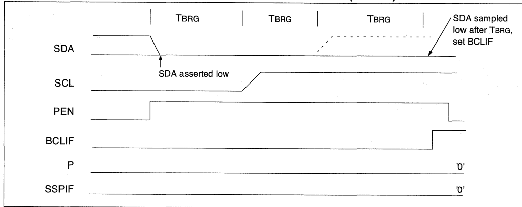
FIGURE 17-26: BUS COLLISION DURING A STOP CONDITION (CASE 1)
