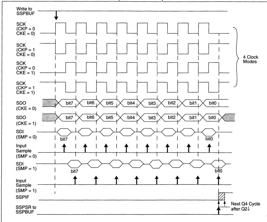
FIGURE 17-2: SPI MODE WAVEFORM (MASTER MODE)
