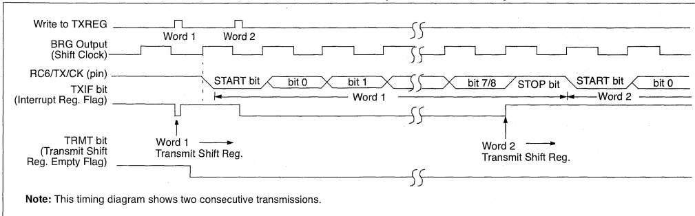
FIGURE 18-3: ASYNCHRONOUS TRANSMISSION (BACK TO BACK)
