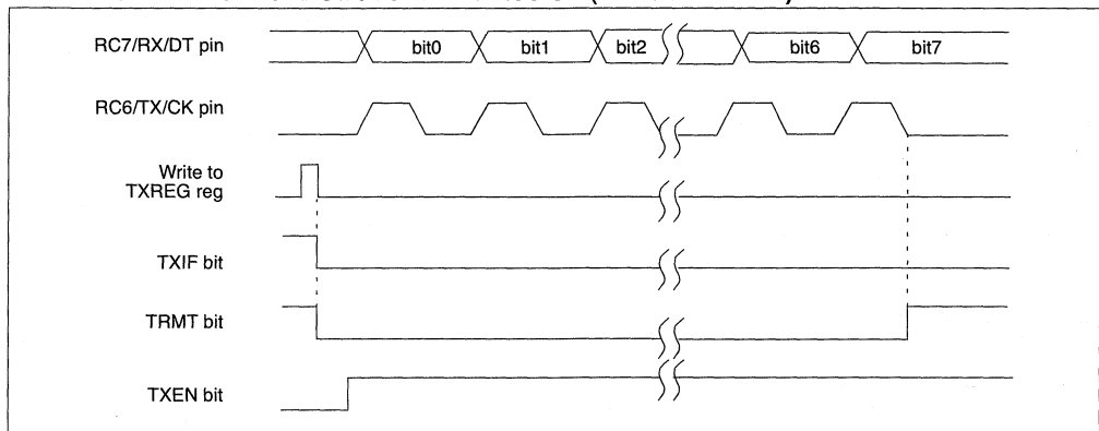
FIGURE 18-7: SYNCHRONOUS TRANSMISSION (THROUGH TXEN)
