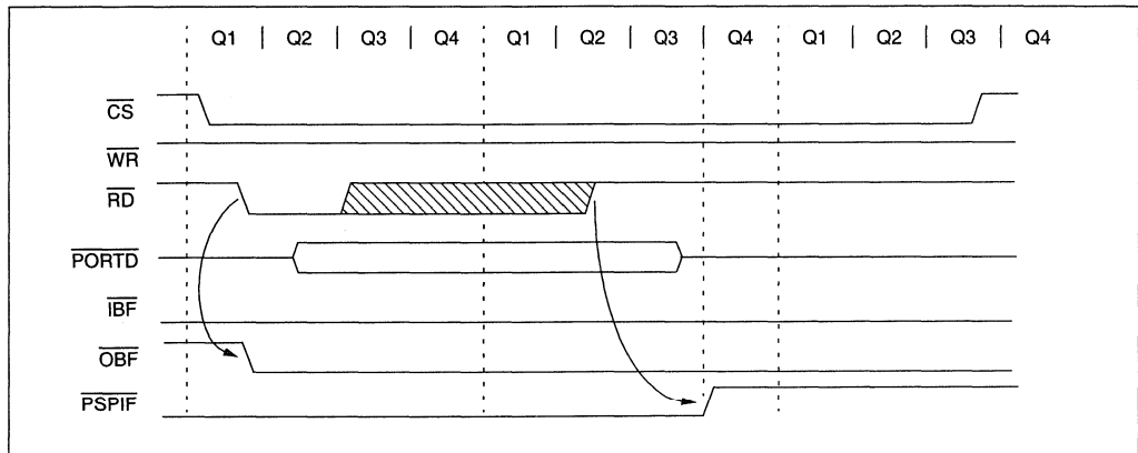
FIGURE 10-3: PARALLEL SLAVE PORT READ WAVEFORMS
