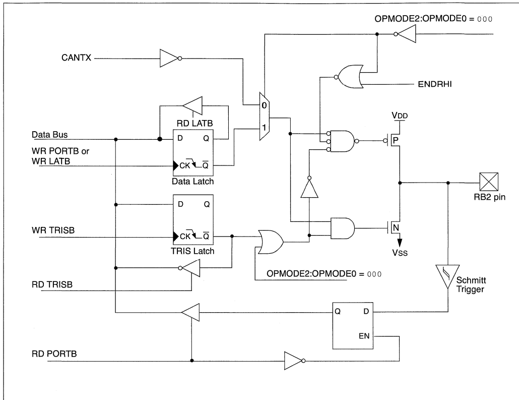
FIGURE 9-6: RB2/CANTX BLOCK DIAGRAM
