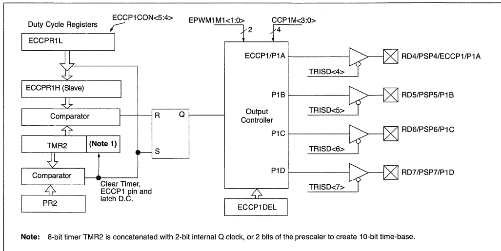
FIGURE 16-3: SIMPLIFIED PWM BLOCK DIAGRAM
