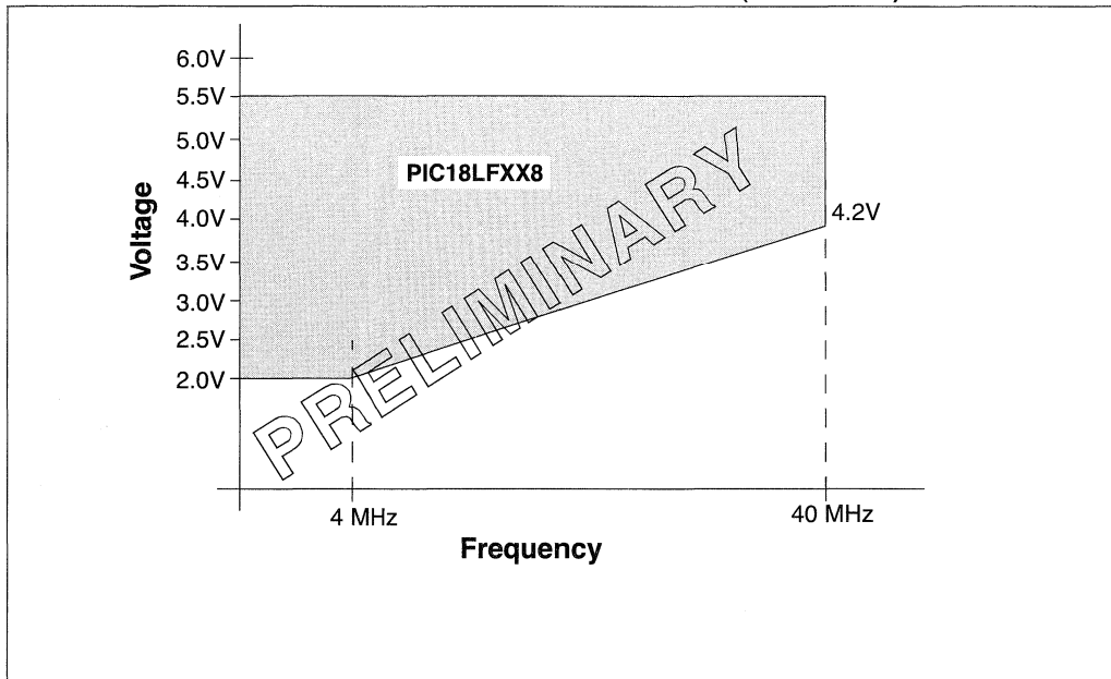
FIGURE 27-2: PIC18LFXX8 VOLTAGE-FREQUENCY GRAPH (INDUSTRIAL)
