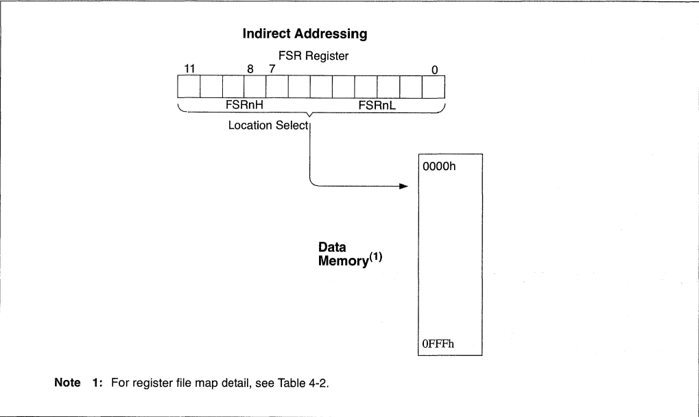
FIGURE 4-8: INDIRECT ADDRESSING
