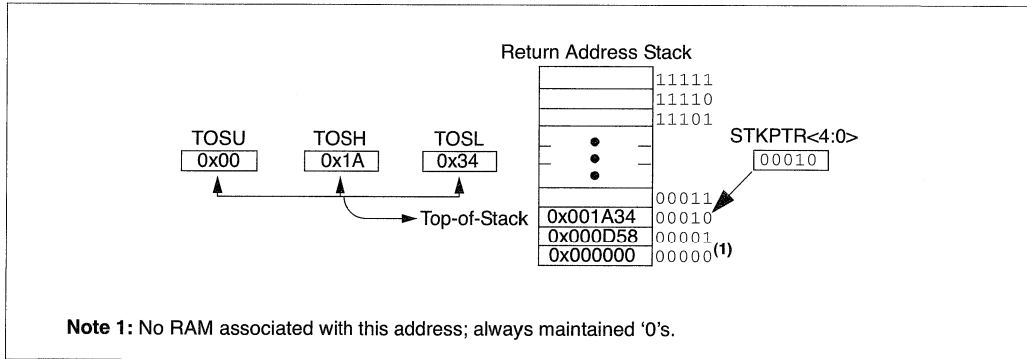
FIGURE 4-3: RETURN ADDRESS STACK AND ASSOCIATED REGISTERS
