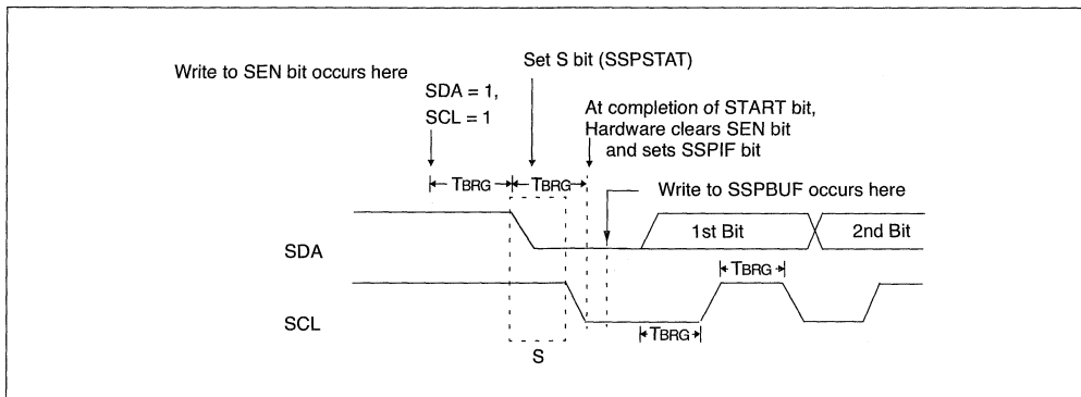
FIGURE 17-13: FIRST START BIT TIMING
