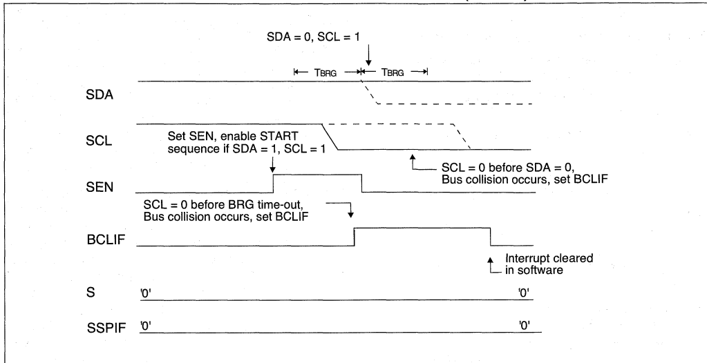
FIGURE 17-22: BUS COLLISION DURING START CONDITION (SCL = 0)
