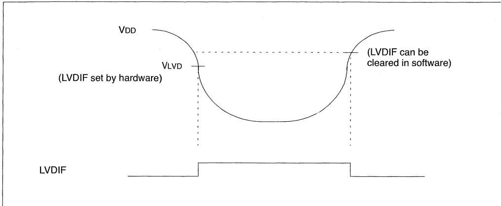
FIGURE 27-3: LOW VOLTAGE DETECT CHARACTERISTICS
