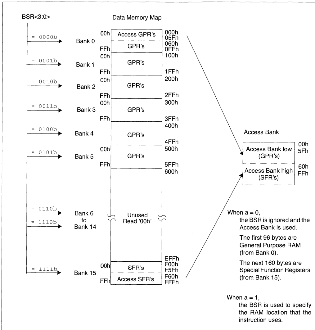
FIGURE 4-5: DATA MEMORY MAP FOR PIC18F258/458
