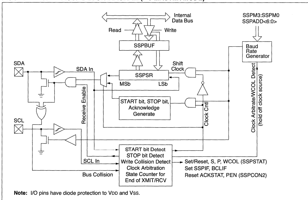
FIGURE 17-10: MSSP BLOCK DIAGRAM (I 2 C MASTER MODE)
