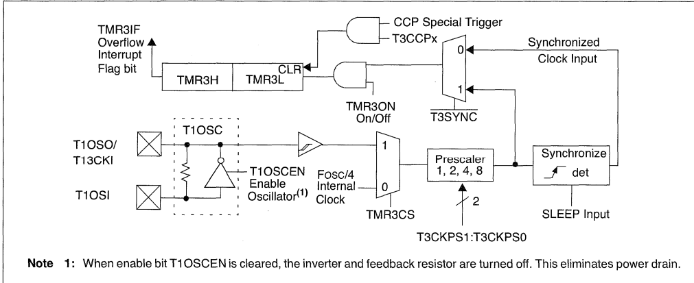
FIGURE 14-1: TIMER3 BLOCK DIAGRAM
