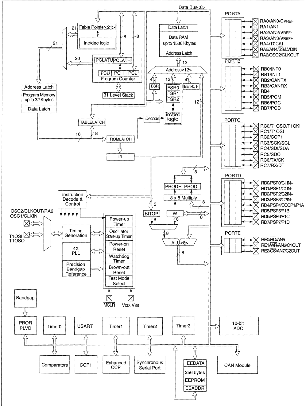
FIGURE 1-2: PIC18F458/448 BLOCK DIAGRAM
