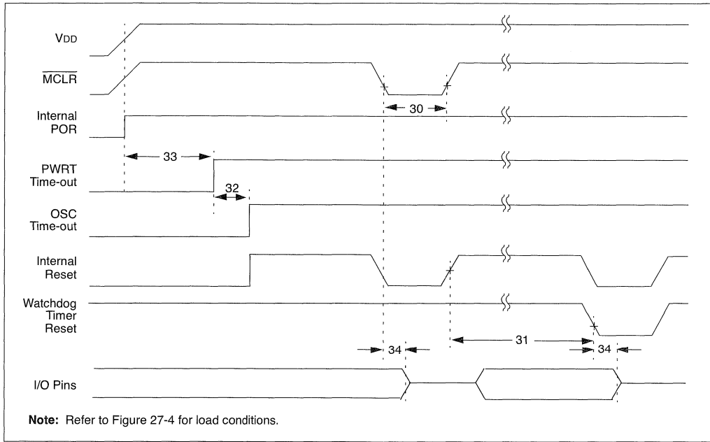
FIGURE 27-7: RESET, WATCHDOG TIMER, OSCILLATOR START-UP TIMER AND POWER-UP TIMER TIMING
