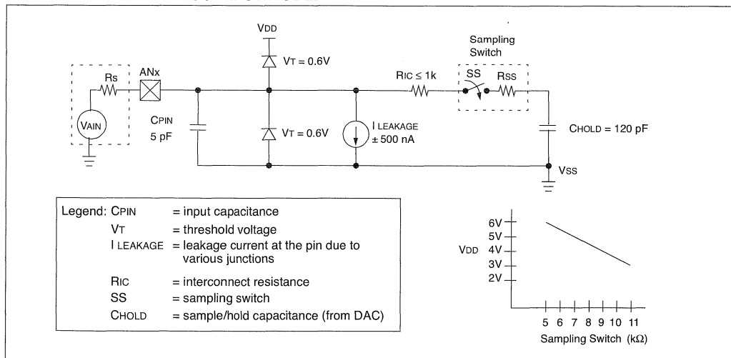
FIGURE 20-2: ANALOG INPUT MODEL
