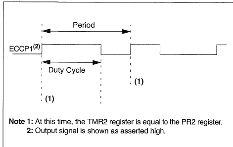
FIGURE 16-4: SINGLE PWM OUTPUT
