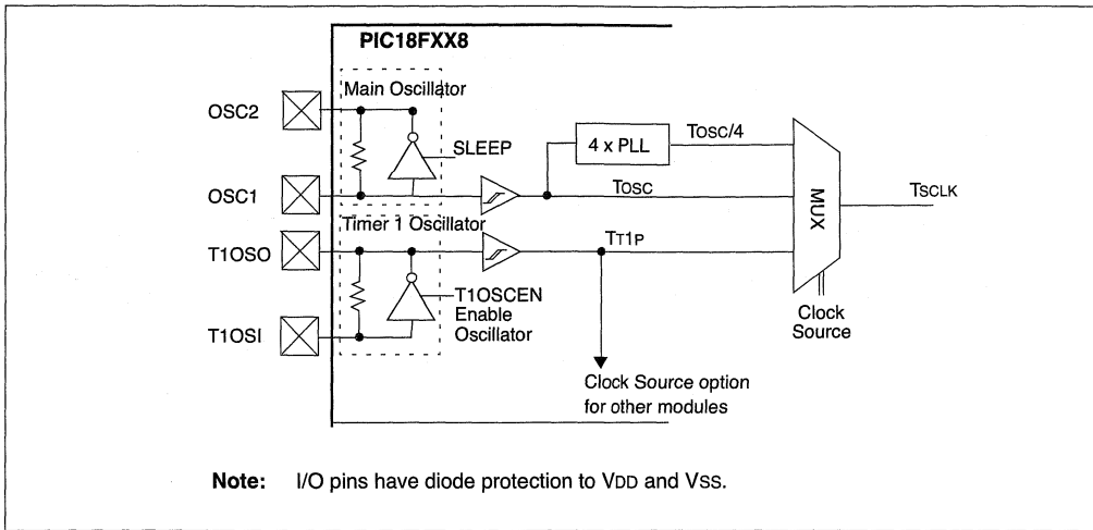
FIGURE 2-6: DEVICE CLOCK SOURCES
