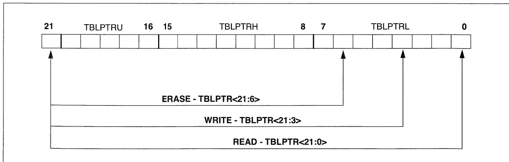
FIGURE 6-3: TABLE POINTER BOUNDARIES BASED ON OPERATION
