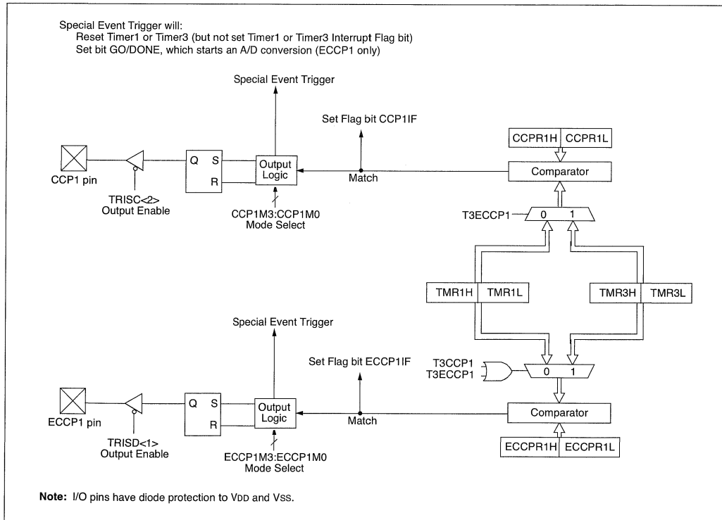
FIGURE 15-2: COMPARE MODE OPERATION BLOCK DIAGRAM
