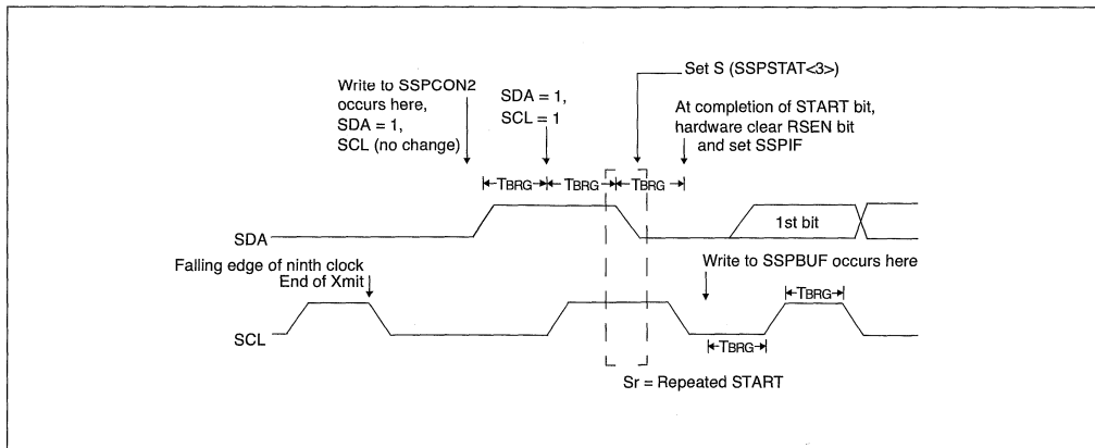
FIGURE 17-14: REPEAT START CONDITION WAVEFORM
