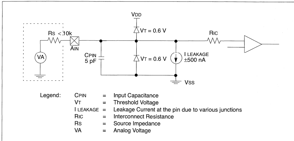
FIGURE 21-4: ANALOG INPUT MODEL
