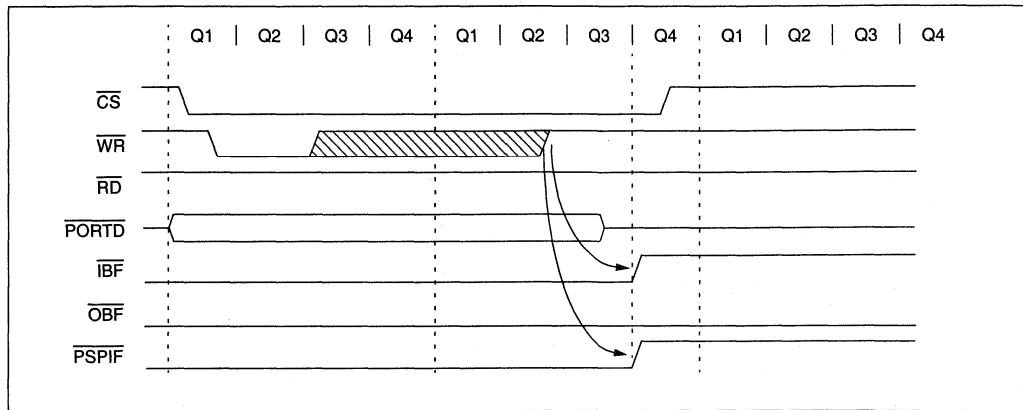
FIGURE 10-2: PARALLEL SLAVE PORT WRITE WAVEFORMS
