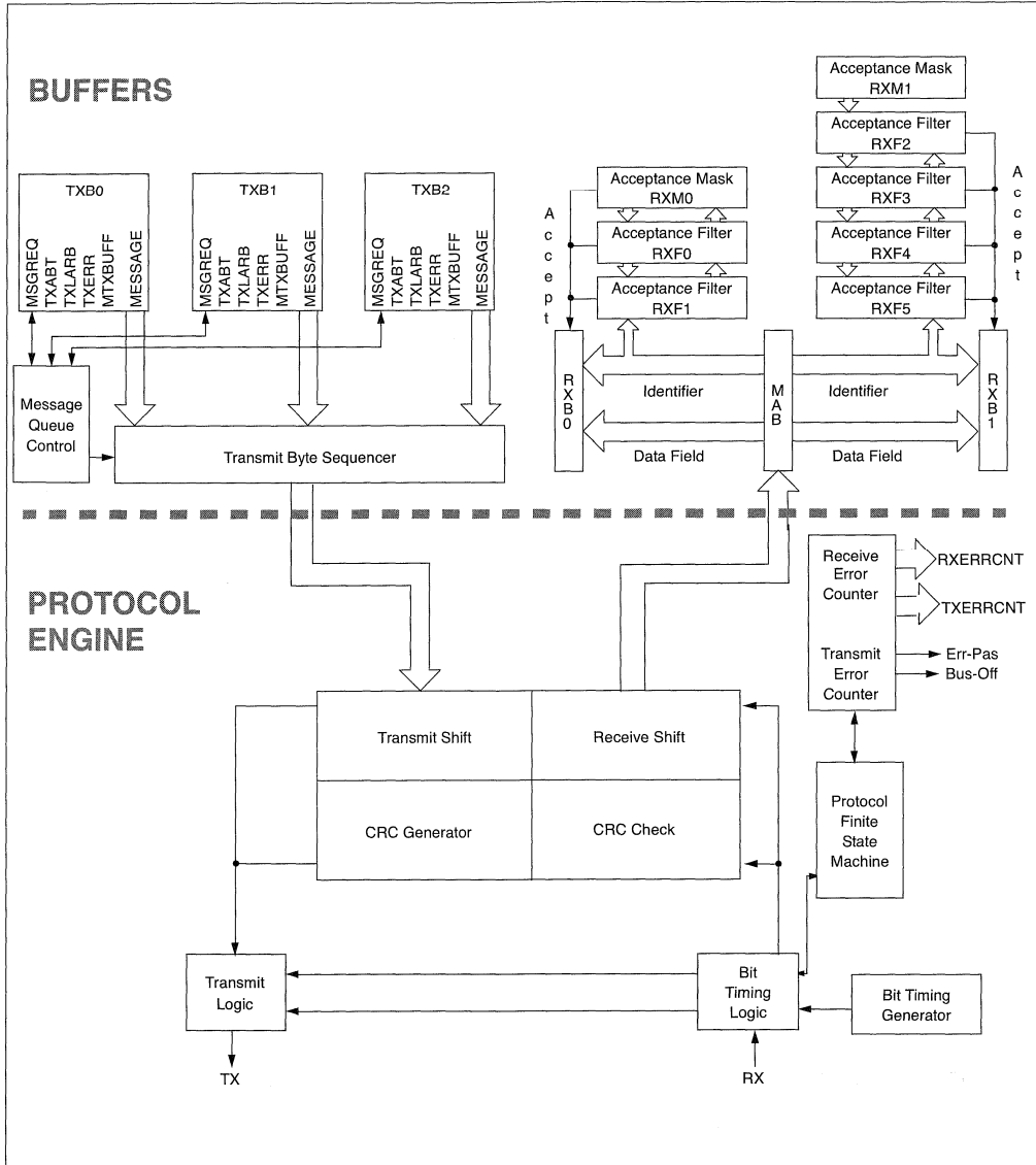
FIGURE 19-1: CAN BUFFERS AND PROTOCOL ENGINE BLOCK DIAGRAM
