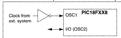
FIGURE 2-4: EXTERNAL CLOCK INPUT OPERATION (ECIO CONFIGURATION)
