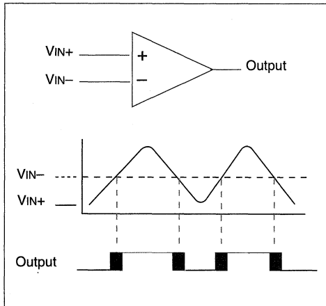
FIGURE 21-2: SINGLE COMPARATOR
