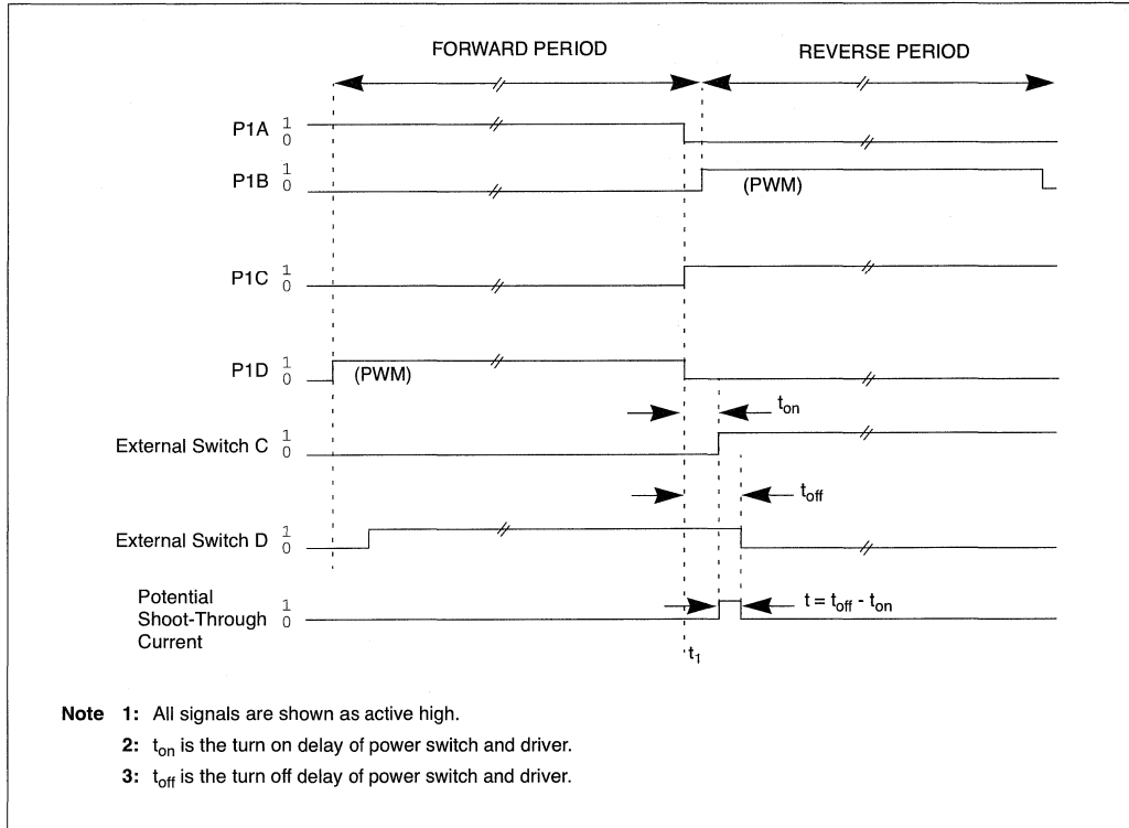
FIGURE 16-11: PWM DIRECTION CHANGE AT NEAR 100% DUTY CYCLE
