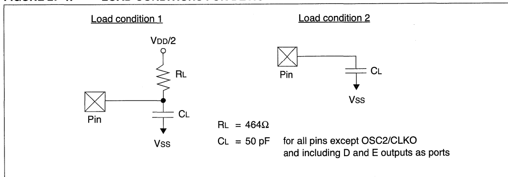
FIGURE 27-4: LOAD CONDITIONS FOR DEVICE TIMING SPECIFICATIONS
