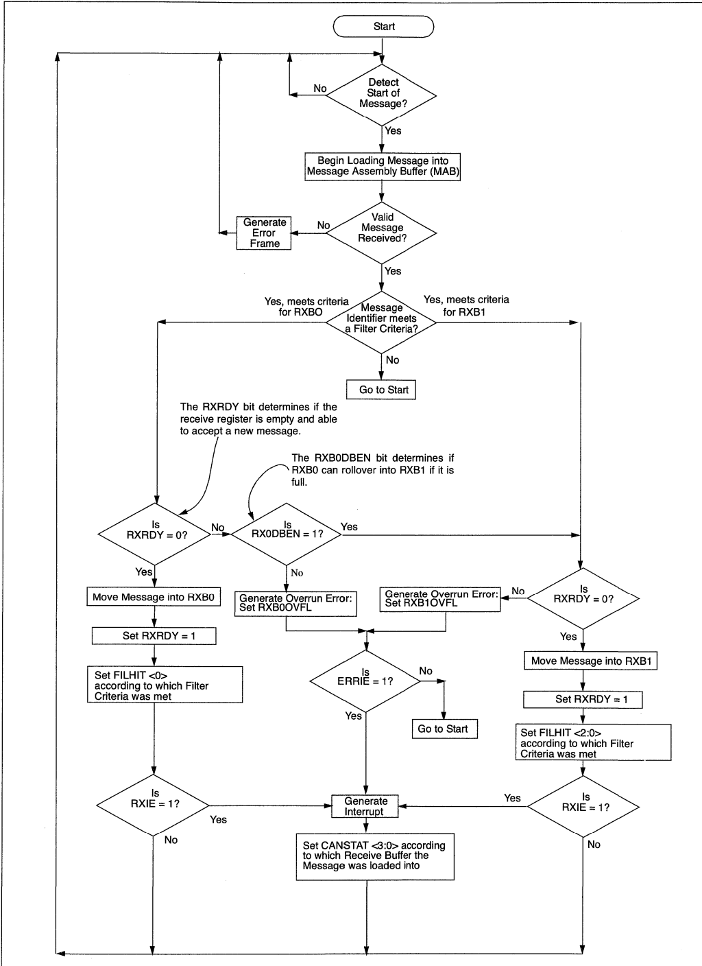
FIGURE 19-4: MESSAGE RECEPTION FLOW CHART
