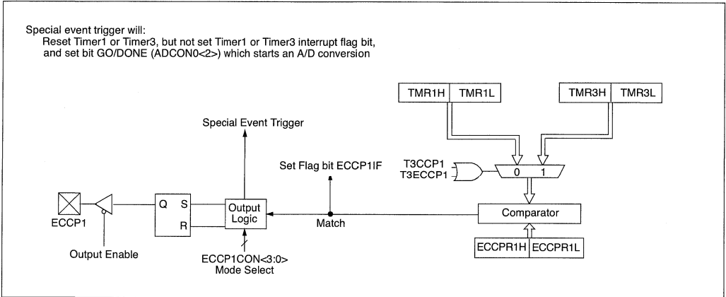
FIGURE 16-2: COMPARE MODE OPERATION BLOCK DIAGRAM
