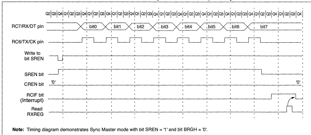
FIGURE 18-8: SYNCHRONOUS RECEPTION (MASTER MODE, SREN)
