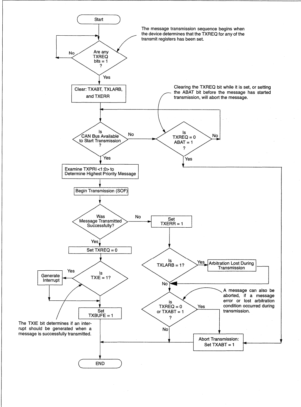
FIGURE 19-2: TRANSMIT MESSAGE FLOW CHART
