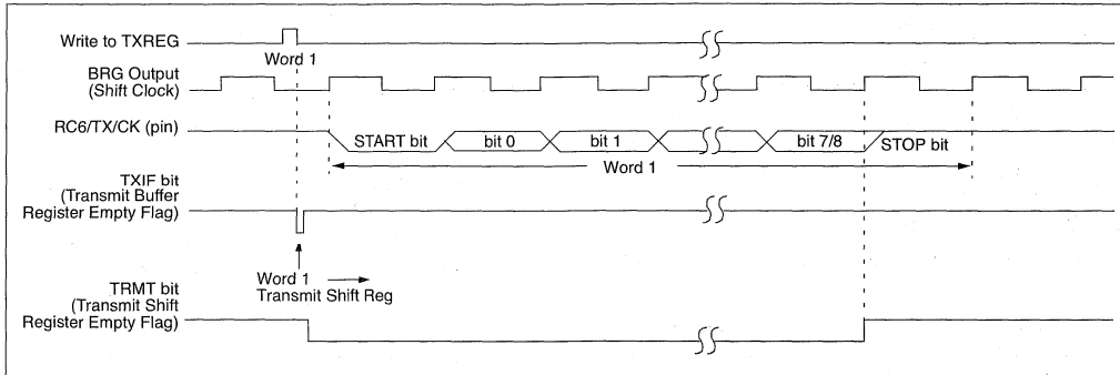
FIGURE 18-2: ASYNCHRONOUS TRANSMISSION
