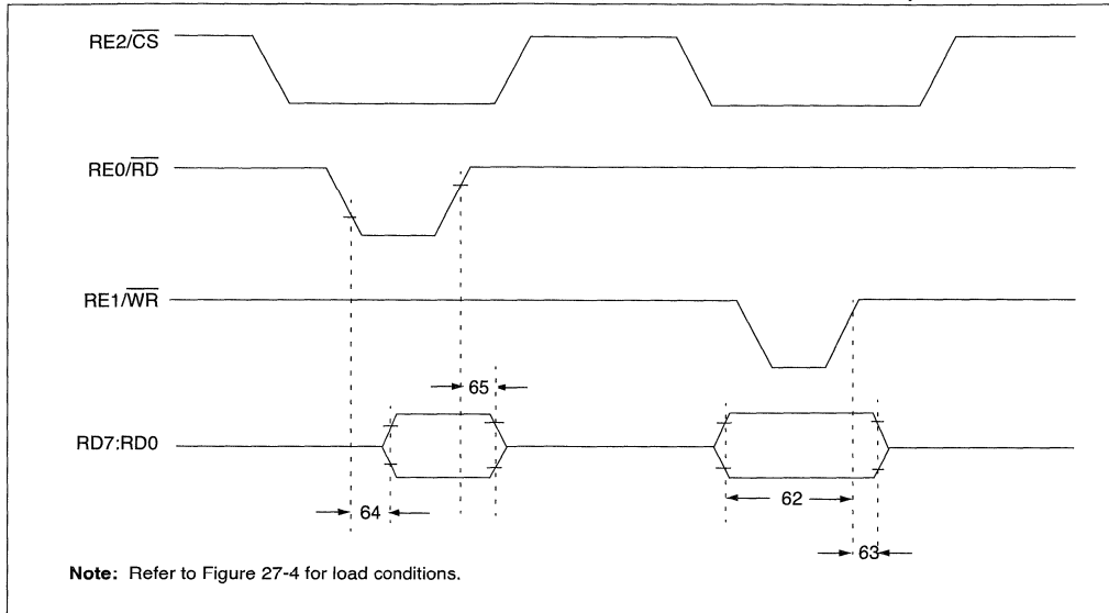
FIGURE 27-11: PARALLEL SLAVE PORT TIMING (PIC18F248 AND PIC18F458)
