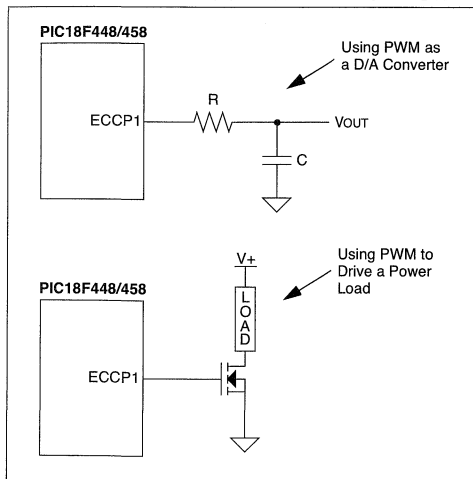
FIGURE 16-5: EXAMPLE OF SINGLE OUTPUT APPLICATION
