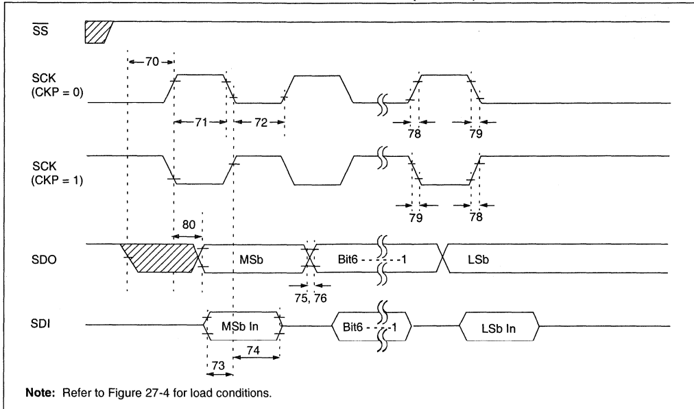
FIGURE 27-12: EXAMPLE SPI MASTER MODE TIMING (CKE = 0)
