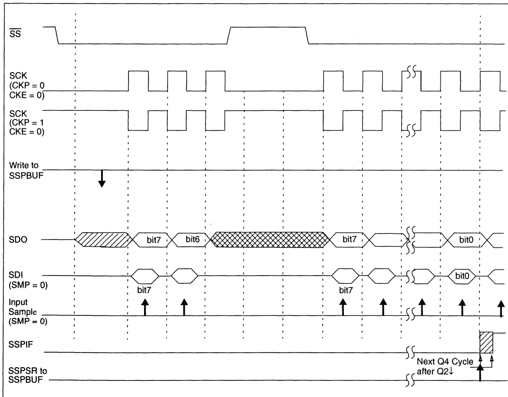
FIGURE 17-3: SLAVE SYNCHRONIZATION WAVEFORM
