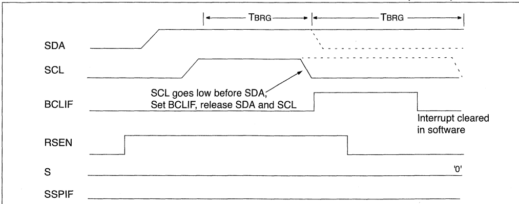
FIGURE 17-25: BUS COLLISION DURING REPEATED START CONDITION (CASE 2)
