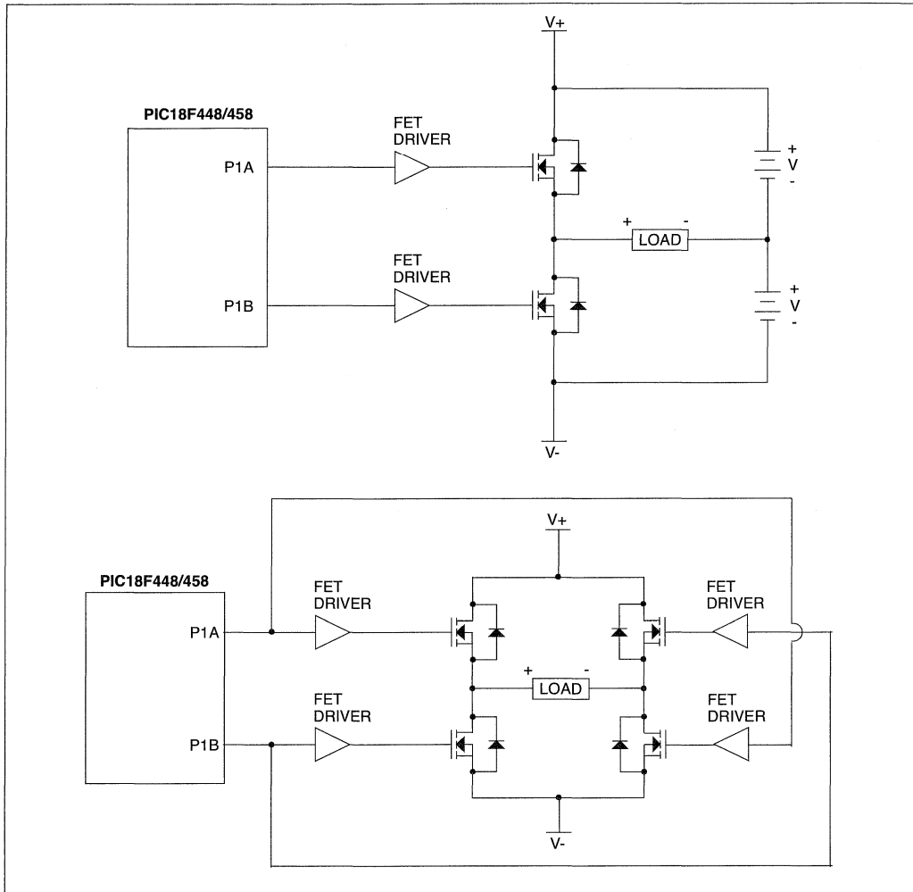
FIGURE 16-7: EXAMPLE OF HALF-BRIDGE OUTPUT MODE APPLICATIONS
