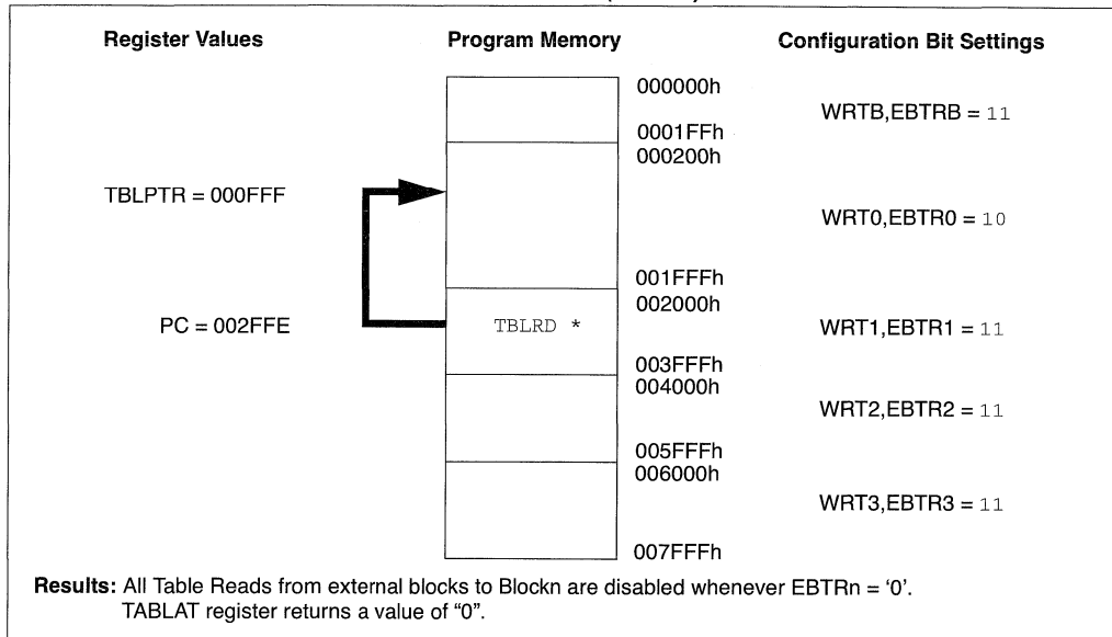
FIGURE 24-5: EXTERNAL BLOCK TABLE READ (EBTRn) DISALLOWED
