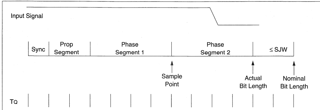
FIGURE 19-8: SHORTENING A BIT PERIOD
