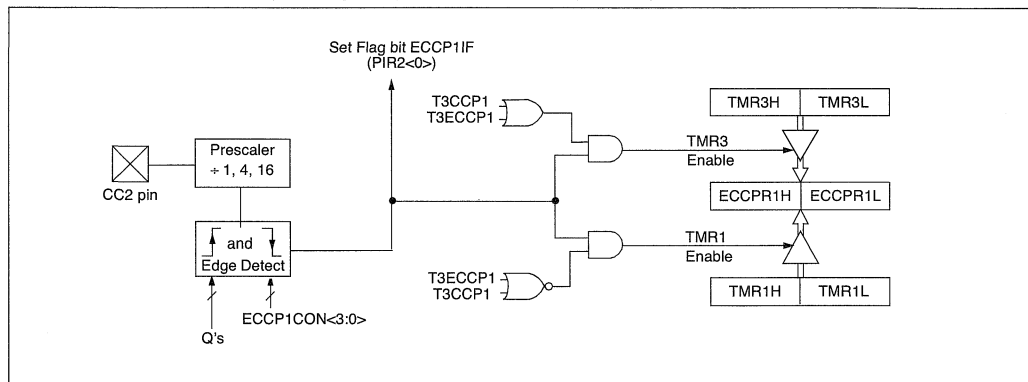
FIGURE 16-1: CAPTURE MODE OPERATION BLOCK DIAGRAM
