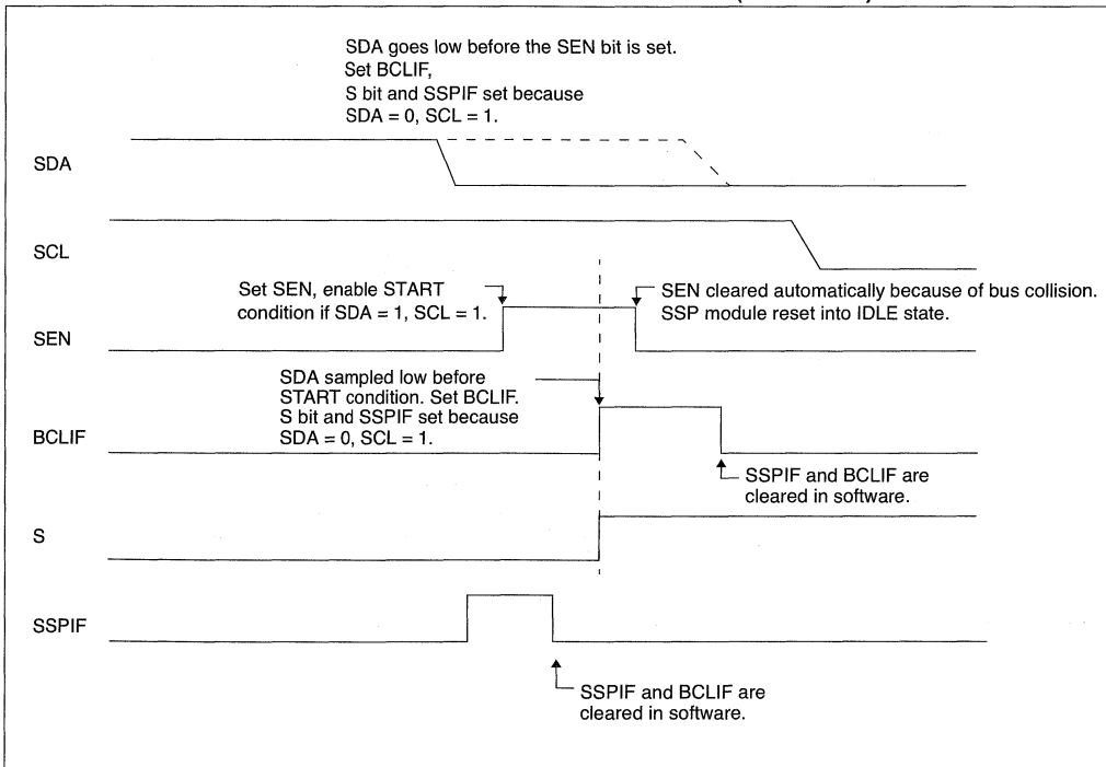
FIGURE 17-21: BUS COLLISION DURING START CONDITION (SDA ONLY)
