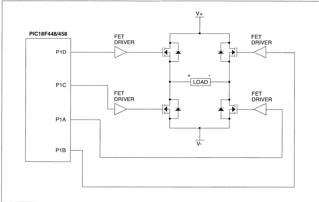
FIGURE 16-9: EXAMPLE OF FULL-BRIDGE APPLICATION
