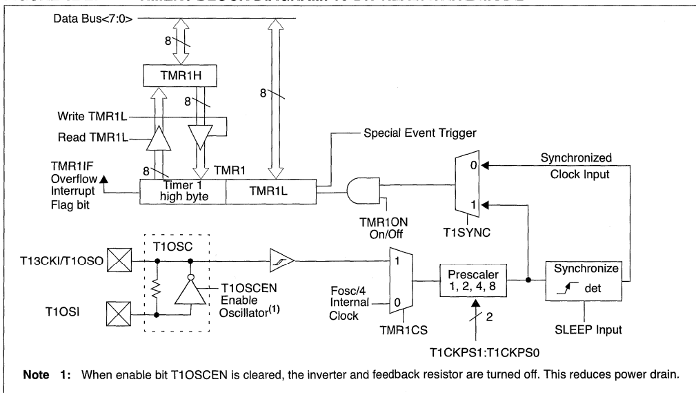
FIGURE 12-2: TIMER1 BLOCK DIAGRAM: 16-BIT READ/WRITE MODE
