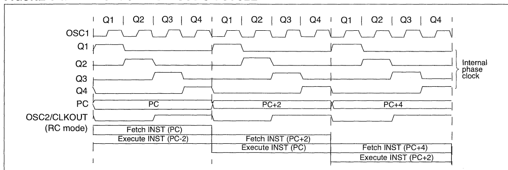
FIGURE 4-4: CLOCK/INSTRUCTION CYCLE
