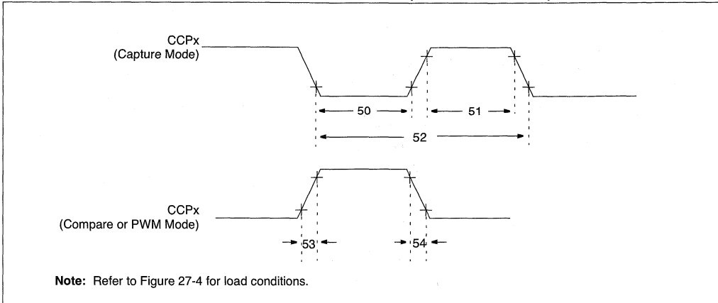
FIGURE 27-10: CAPTURE/COMPARE/PWM TIMINGS (CCP1 AND ECCP1)
