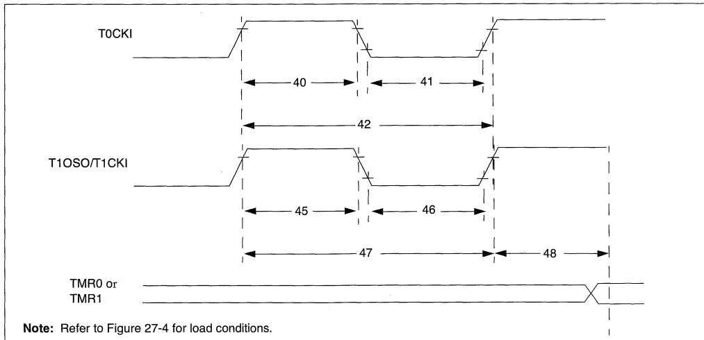
FIGURE 27-9: TIMER0 AND TIMER1 EXTERNAL CLOCK TIMINGS
