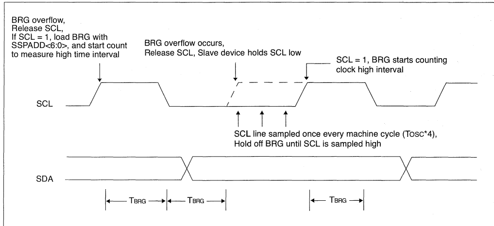
FIGURE 17-19: CLOCK ARBITRATION TIMING IN MASTER TRANSMIT MODE
