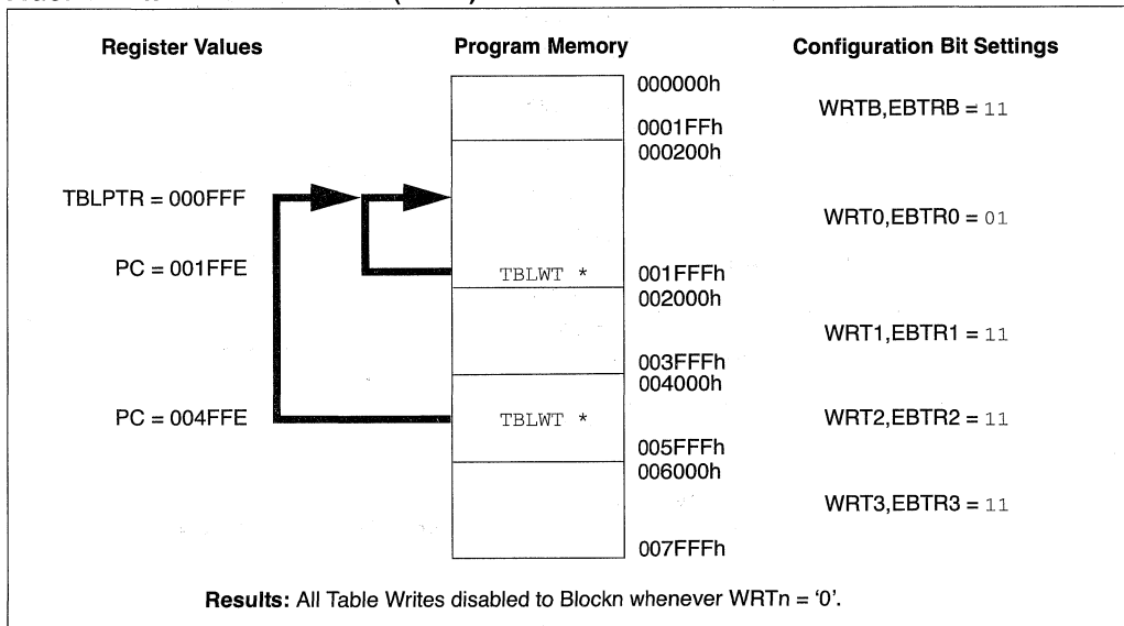
FIGURE 24-4: TABLE WRITE (WRTn) DISALLOWED
