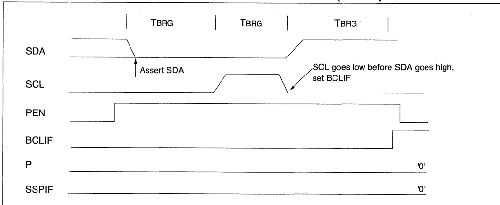
FIGURE 17-27: BUS COLLISION DURING A STOP CONDITION (CASE 2)
