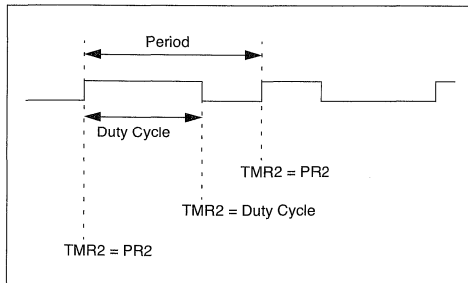
FIGURE 15-4: PWM OUTPUT
