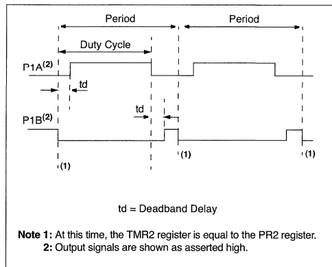
FIGURE 16-6: HALF-BRIDGE PWM OUTPUT
