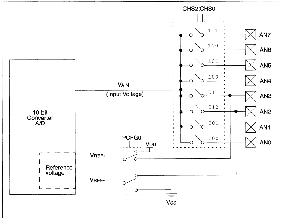
FIGURE 20-1: A/D BLOCK DIAGRAM
