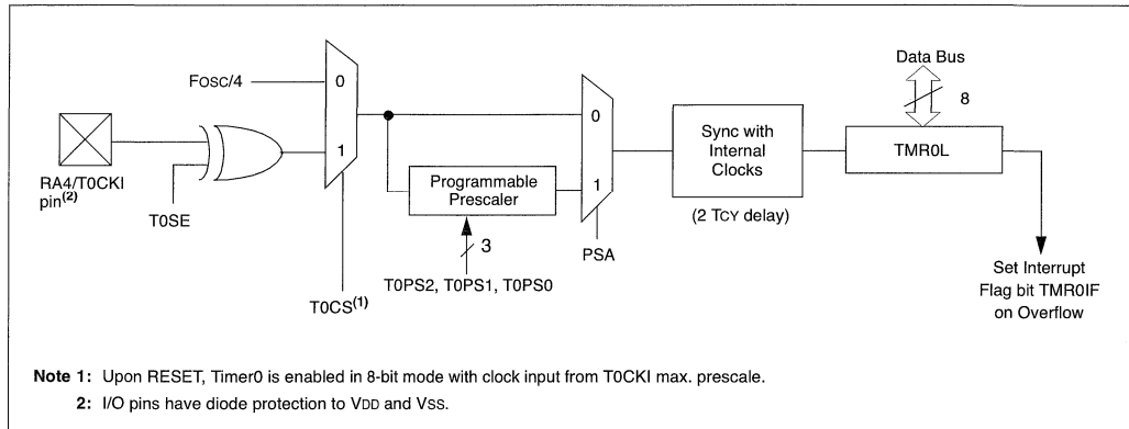
FIGURE 11-1: TIMER0 BLOCK DIAGRAM IN 8-BIT MODE
