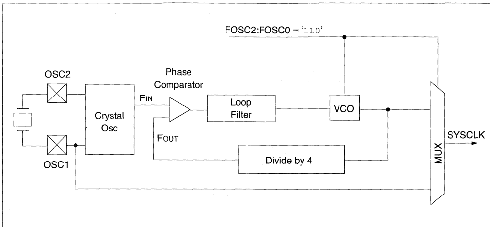
FIGURE 2-5: PLL BLOCK DIAGRAM
