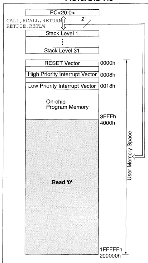
FIGURE 4-2: PROGRAM MEMORY MAP AND STACK FOR PIC18F248/448
