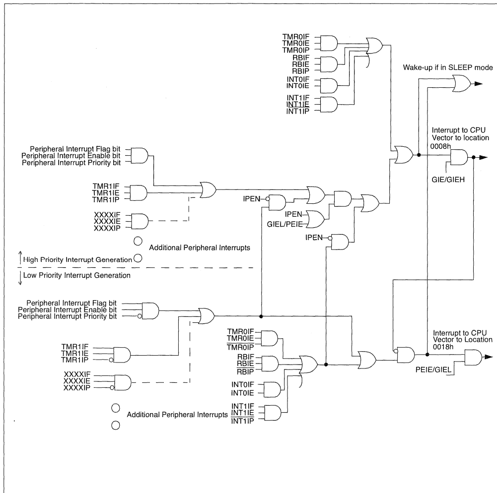
FIGURE 8-1: INTERRUPT LOGIC
