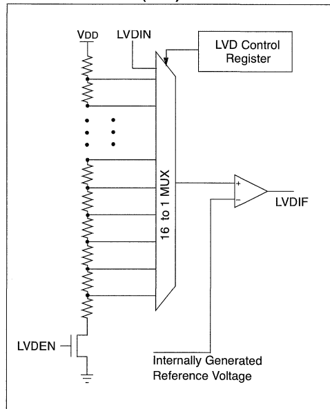
FIGURE 23-2: LOW VOLTAGE DETECT (LVD) BLOCK DIAGRAM
