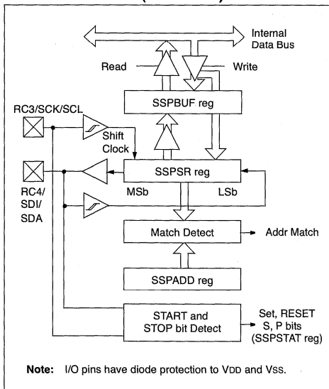
FIGURE 17-6: MSSP BLOCK DIAGRAM (I 2 C MODE)
