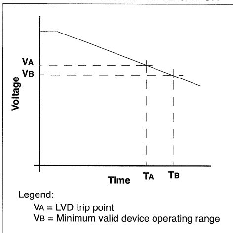
FIGURE 23-1: TYPICAL LOW VOLTAGE DETECT APPLICATION
