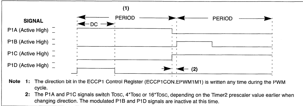
FIGURE 16-10: PWM DIRECTION CHANGE
