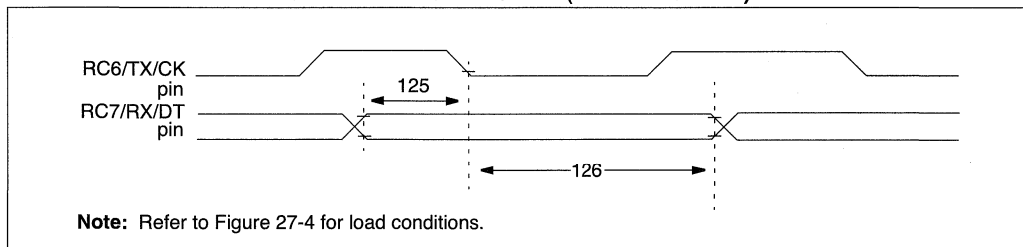
FIGURE 27-21: USART SYNCHRONOUS RECEIVE (MASTER/SLAVE) TIMING
