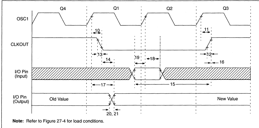
FIGURE 27-6: CLKOUT AND I/O TIMING
