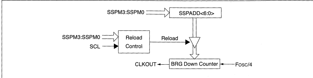
FIGURE 17-11: BAUD RATE GENERATOR BLOCK DIAGRAM
