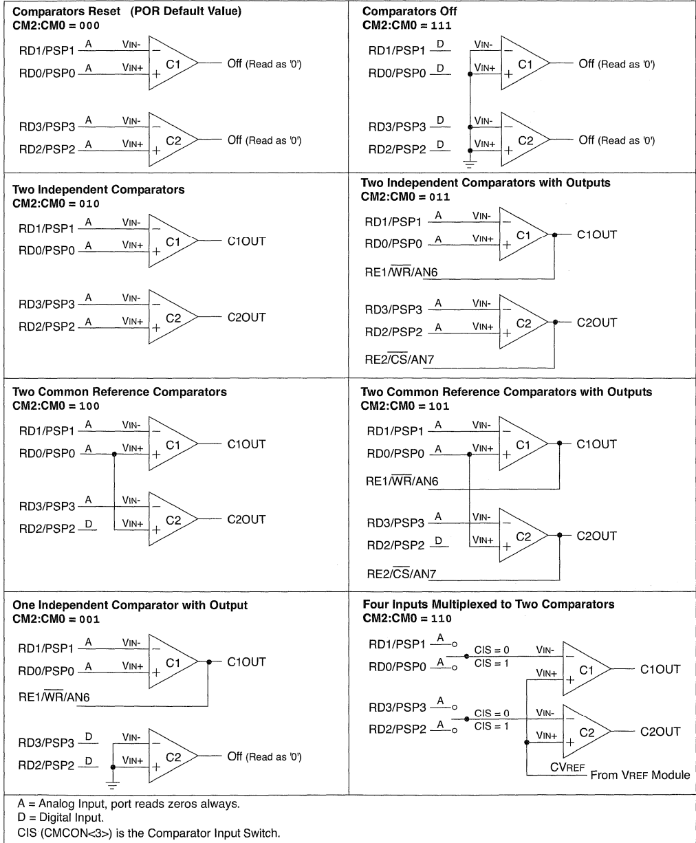
FIGURE 21-1: COMPARATOR I/O OPERATING MODES
