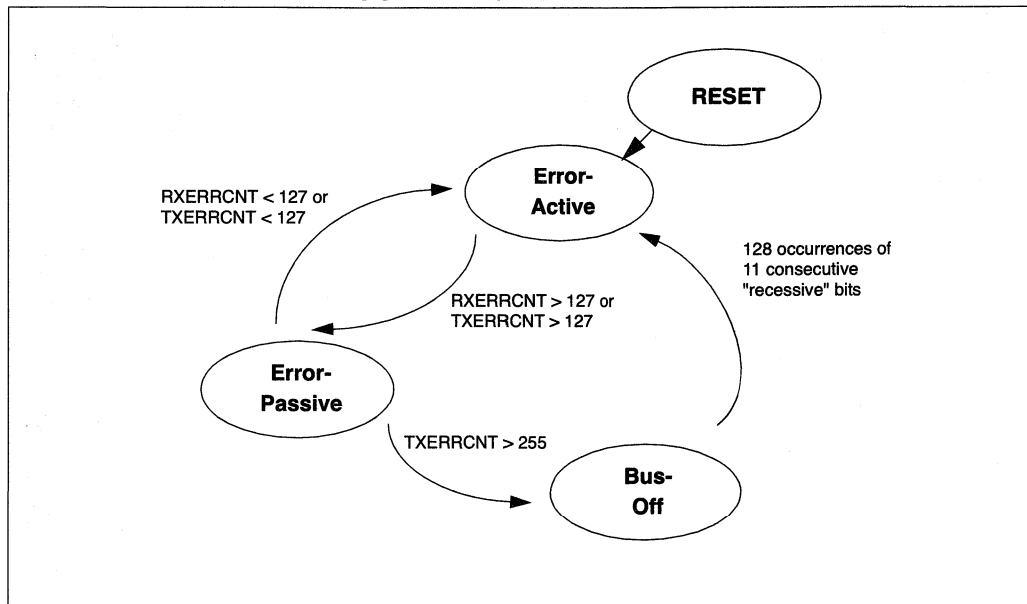
FIGURE 19-9: ERROR MODES STATE DIAGRAM
