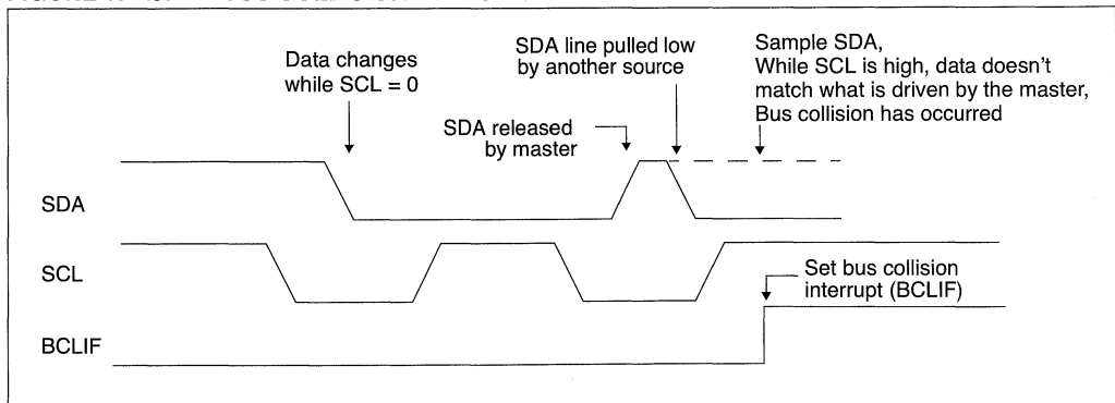
FIGURE 17-20: BUS COLLISION TIMING FOR TRANSMIT AND ACKNOWLEDGE
