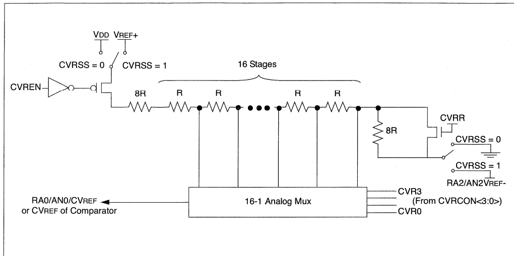
FIGURE 22-1: VOLTAGE REFERENCE BLOCK DIAGRAM
