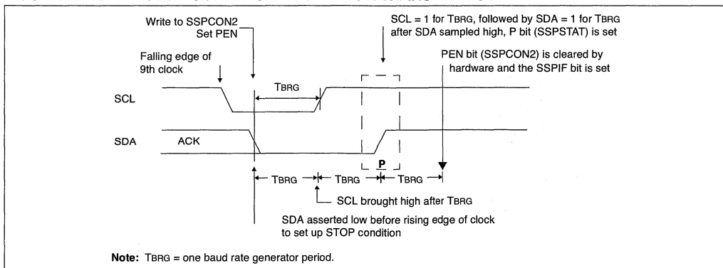
FIGURE 17-18: STOP CONDITION RECEIVE OR TRANSMIT MODE
