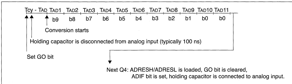
FIGURE 20-3: A/D CONVERSION TAD CYCLES
