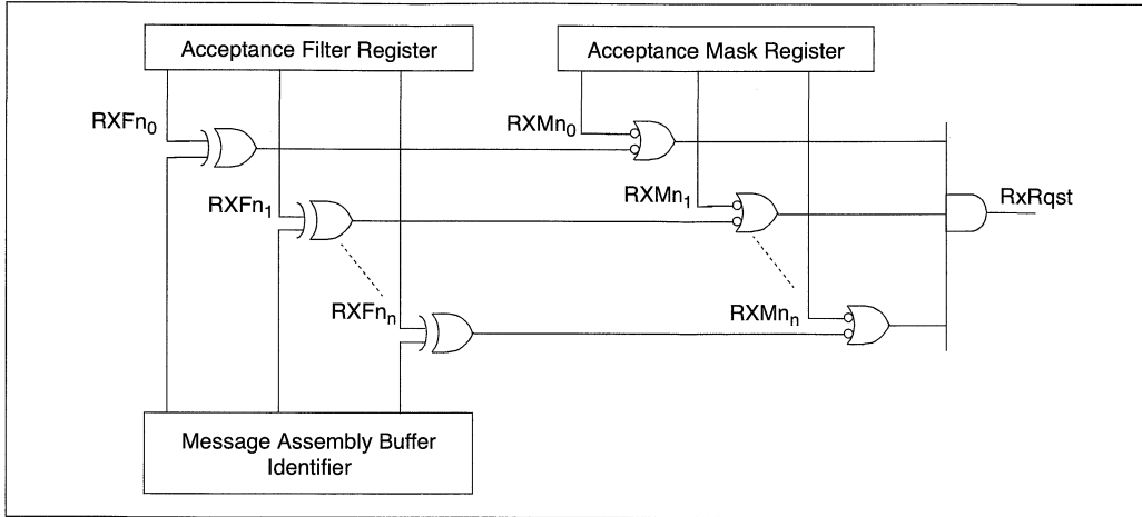
FIGURE 19-5: MESSAGE ACCEPTANCE MASK AND FILTER OPERATION
