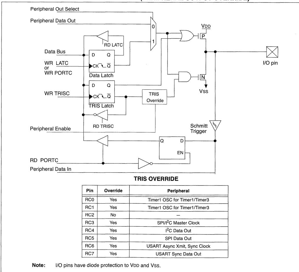
FIGURE 9-8: PORTC BLOCK DIAGRAM (PERIPHERAL OUTPUT OVERRIDE)
