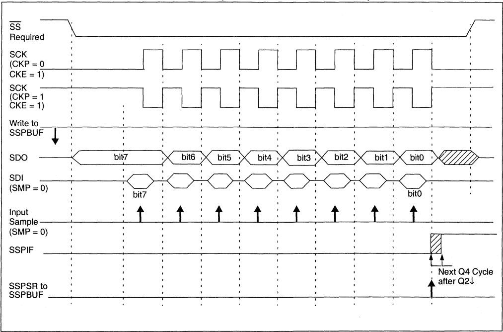
FIGURE 17-5: SPI MODE WAVEFORM (SLAVE MODE WITH CKE = 1)
