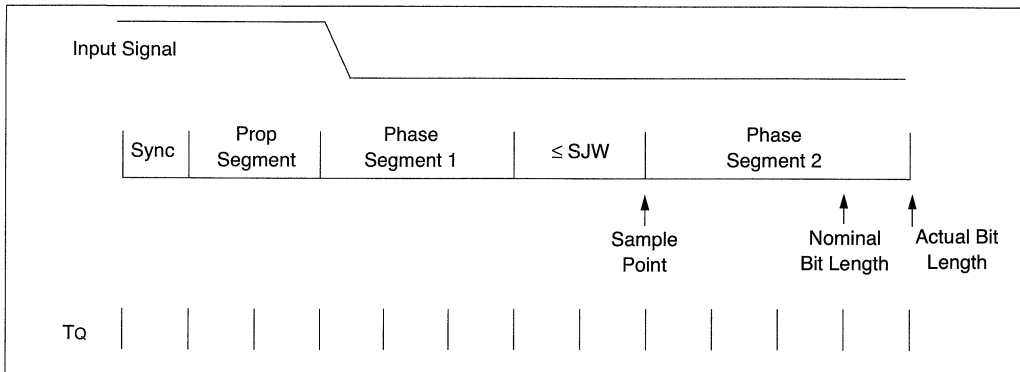
FIGURE 19-7: LENGTHENING A BIT PERIOD
