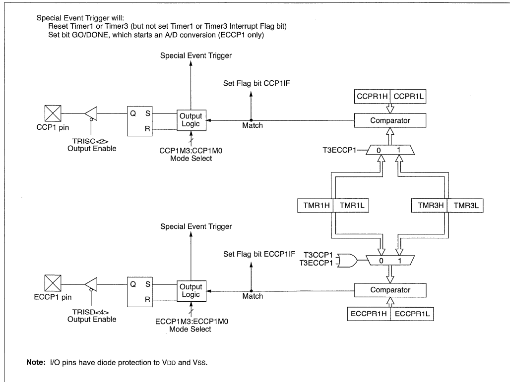
FIGURE 15-1: CAPTURE MODE OPERATION BLOCK DIAGRAM
