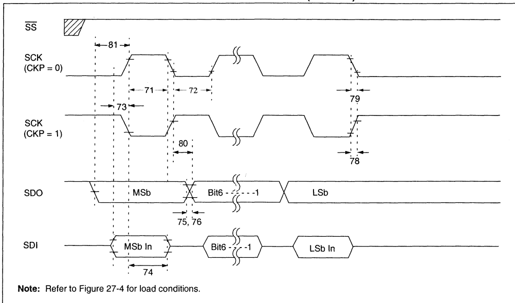
FIGURE 27-13: EXAMPLE SPI MASTER MODE TIMING (CKE = 1)
