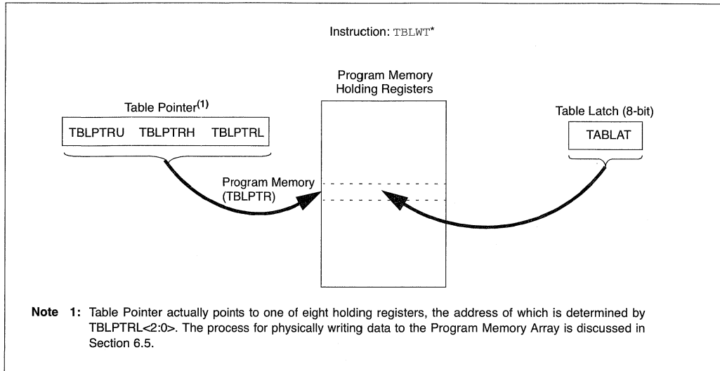
FIGURE 6-2: TABLE WRITE OPERATION
