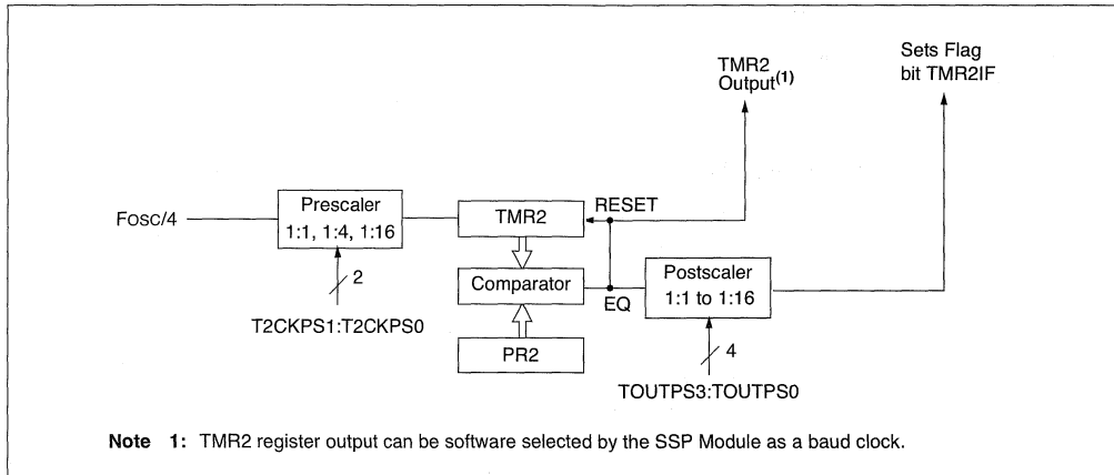
FIGURE 13-1: TIMER2 BLOCK DIAGRAM
