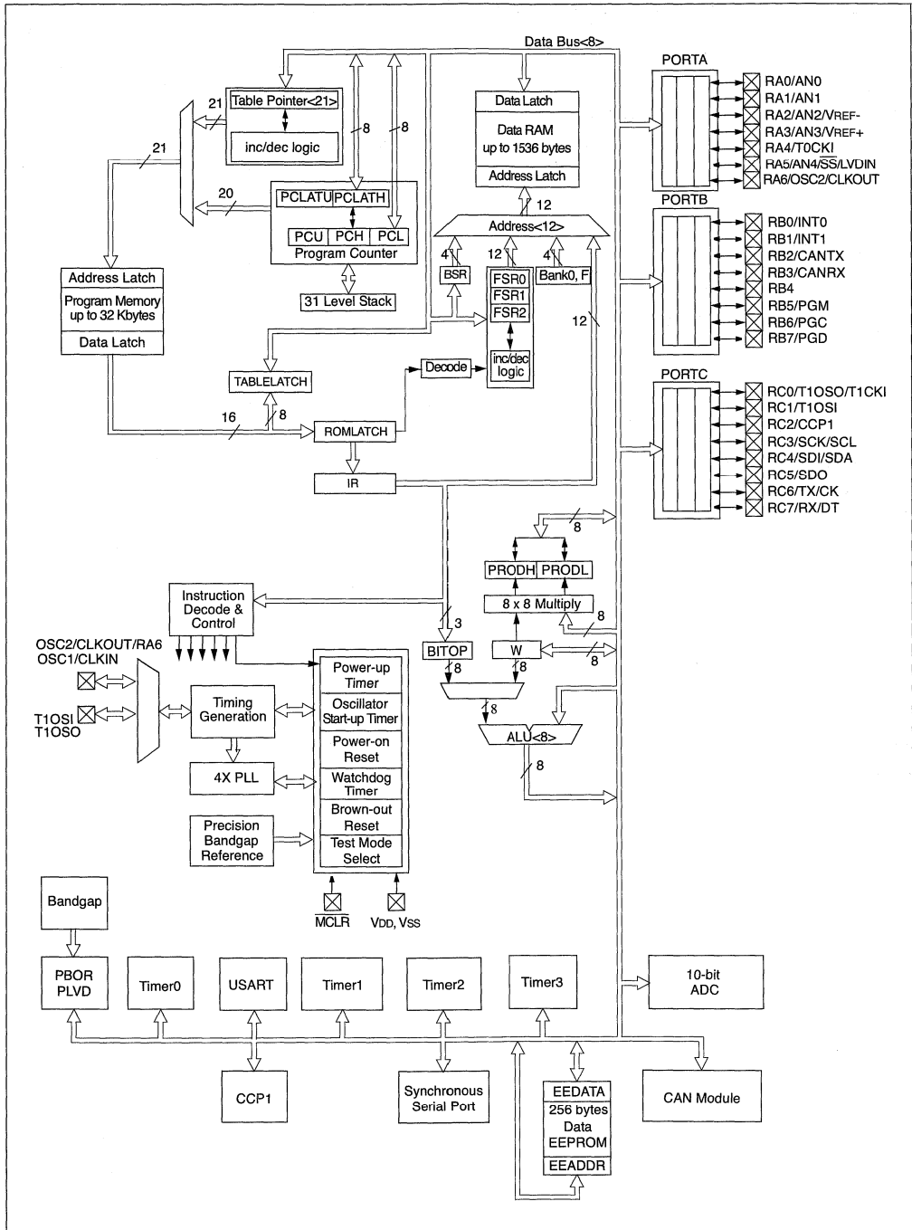
FIGURE 1-1: PIC18F248/258 BLOCK DIAGRAM
