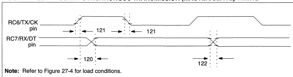
FIGURE 27-20: USART SYNCHRONOUS TRANSMISSION (MASTER/SLAVE) TIMING
