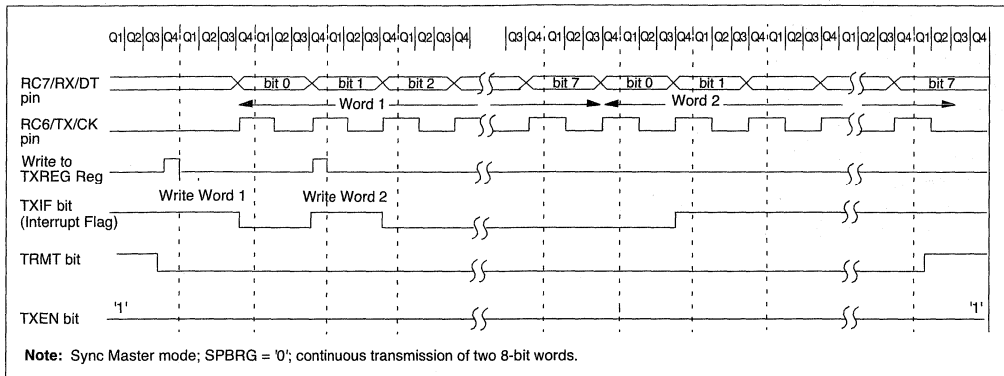
FIGURE 18-6: SYNCHRONOUS TRANSMISSION
