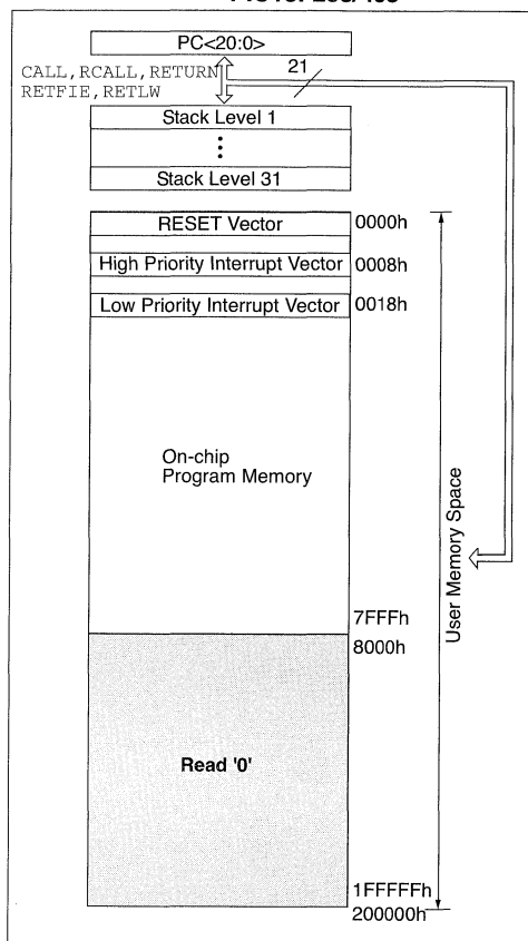
FIGURE 4-1: PROGRAM MEMORY MAP AND STACK FOR PIC18F258/458
