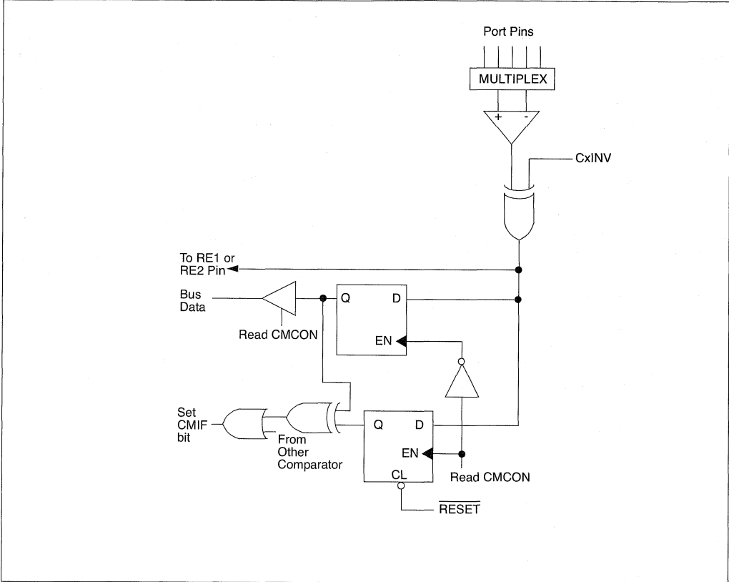
FIGURE 21-3: COMPARATOR OUTPUT BLOCK DIAGRAM
