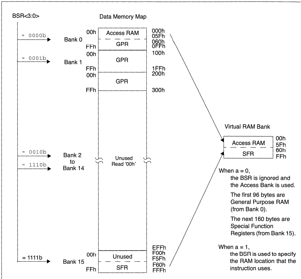
FIGURE 4-6: DATA MEMORY MAP FOR PIC18F248/448
