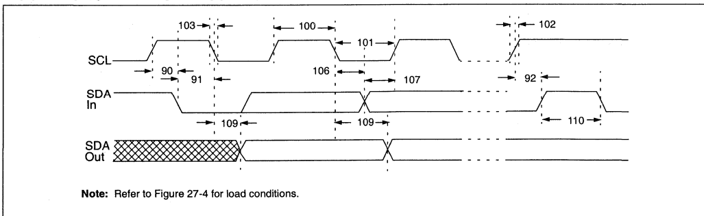
FIGURE 27-19: MASTER SSP I 2 C BUS DATA TIMING
