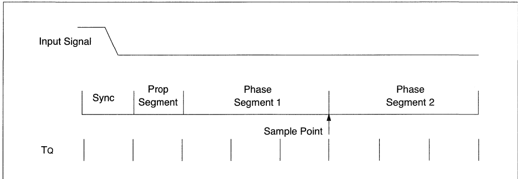
FIGURE 19-6: BIT TIME PARTITIONING
